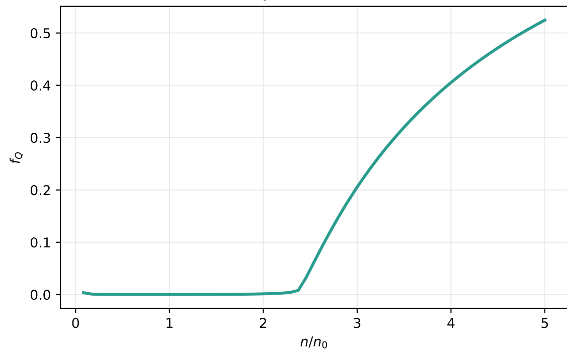
Quark Fraction
