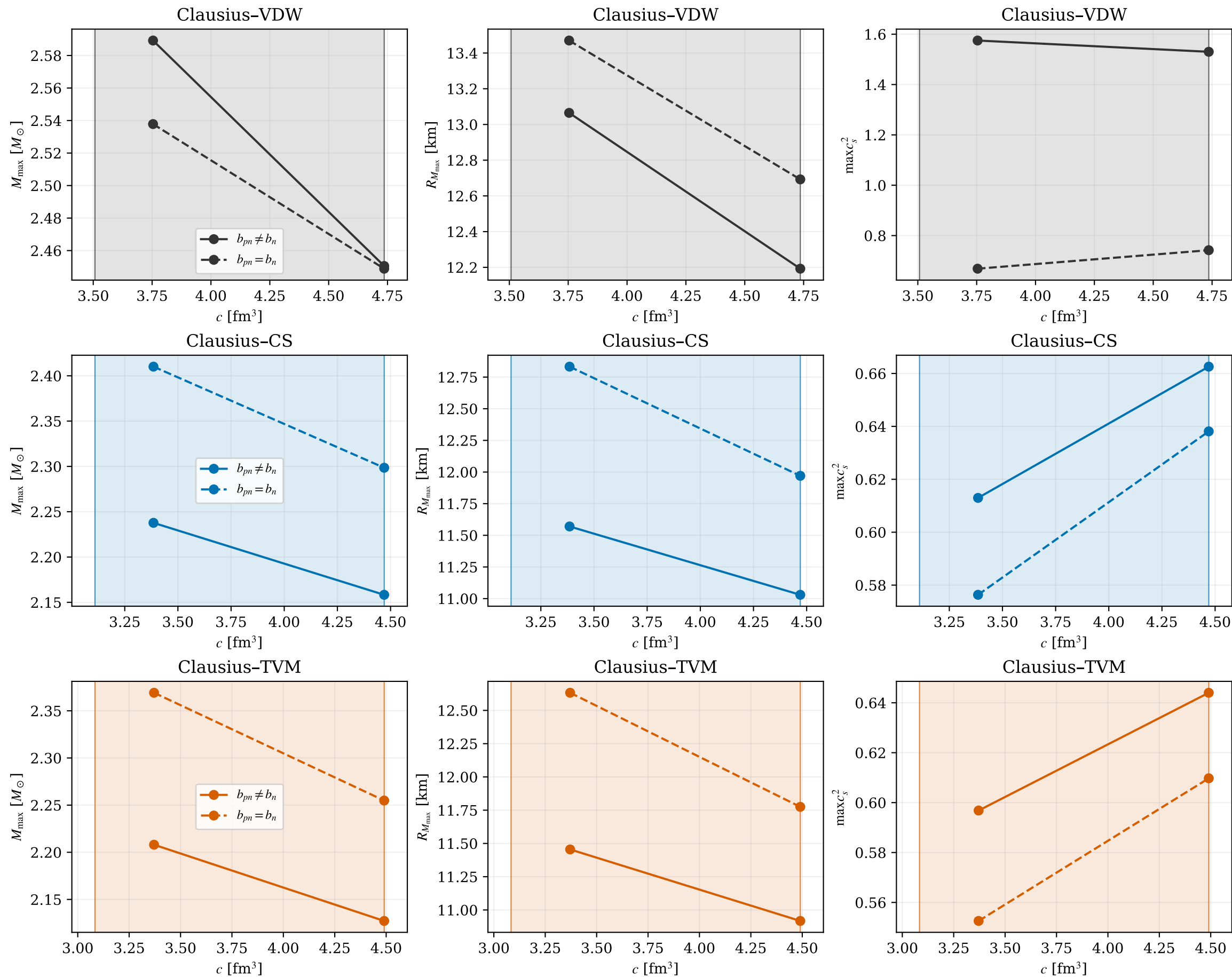
Clausius: empirical parameter bands, 250 \leq K_0 \leq 315 MeV, \Lambda = 300 MeV Shading: calibrated bounds. Markers: saved K_0 = 250, 300 MeV; lines guide the eye.
