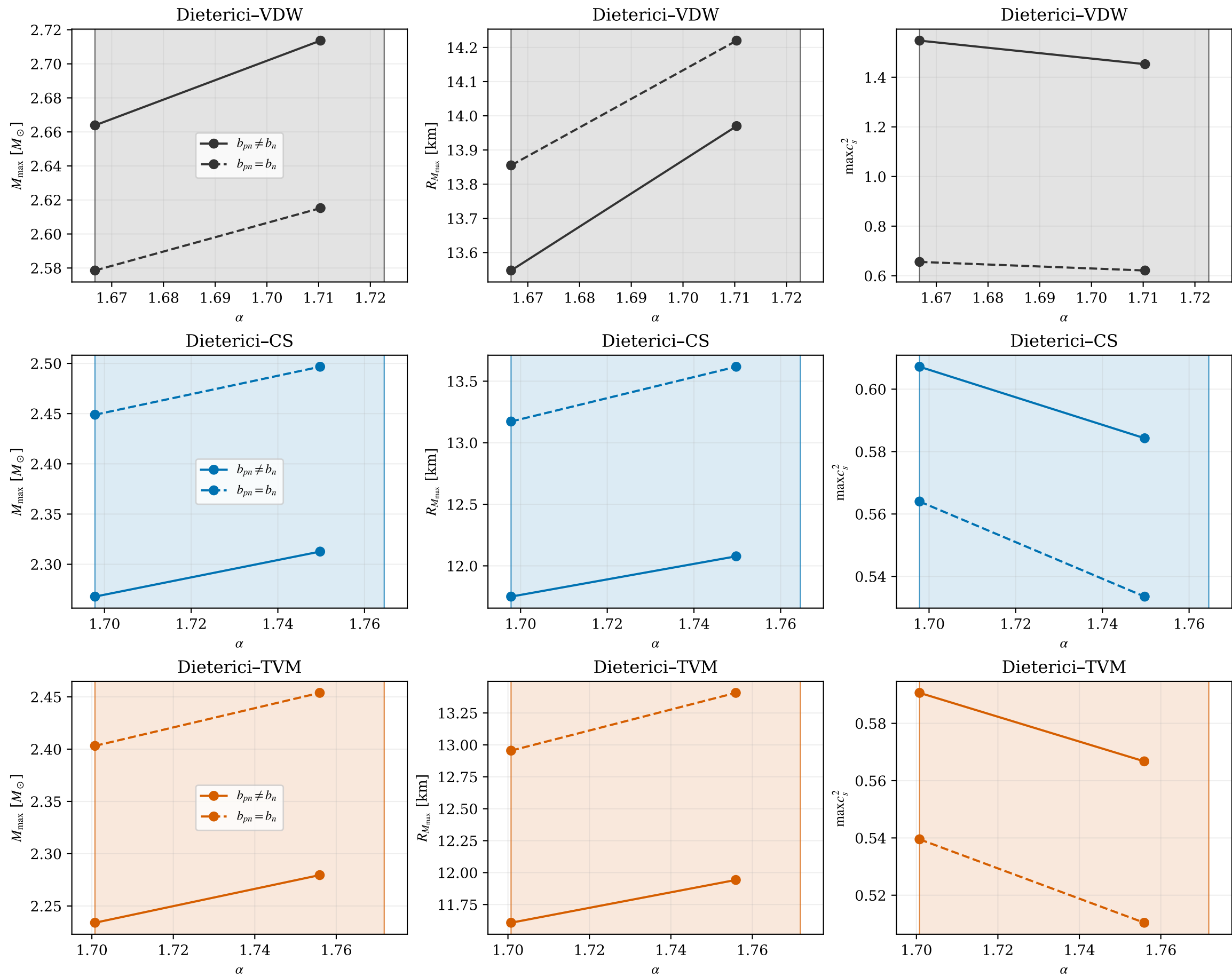
Dieterici: empirical parameter bands, 250 \leq K_0 \leq 315 MeV, \Lambda = 300 MeV Shading: calibrated bounds. Markers: saved K_0 = 250, 300 MeV; lines guide the eye.
