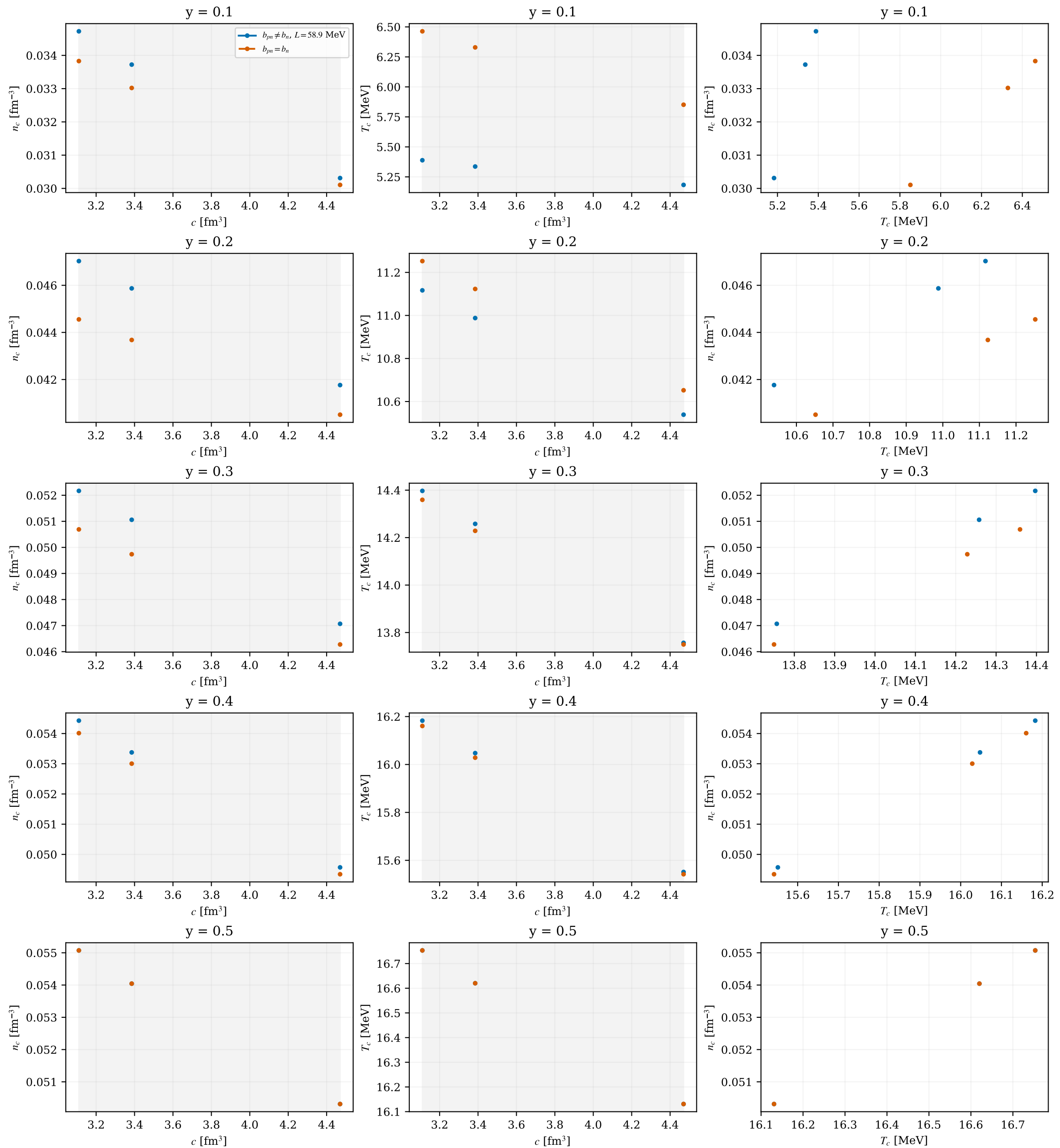
Clausius-CS: fixed-composition critical points (30/140 solved) Gray: empirical parameter interval. Markers: solved points; gaps: missing/failed.
