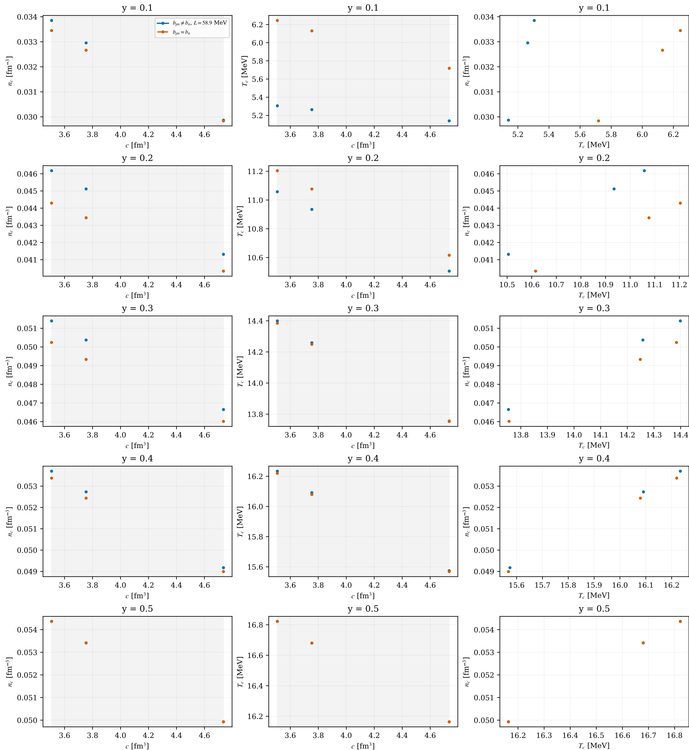
Clausius-VDW: fixed-composition critical points (30/140 solved) Gray: empirical parameter interval. Markers: solved points; gaps: missing/failed.
