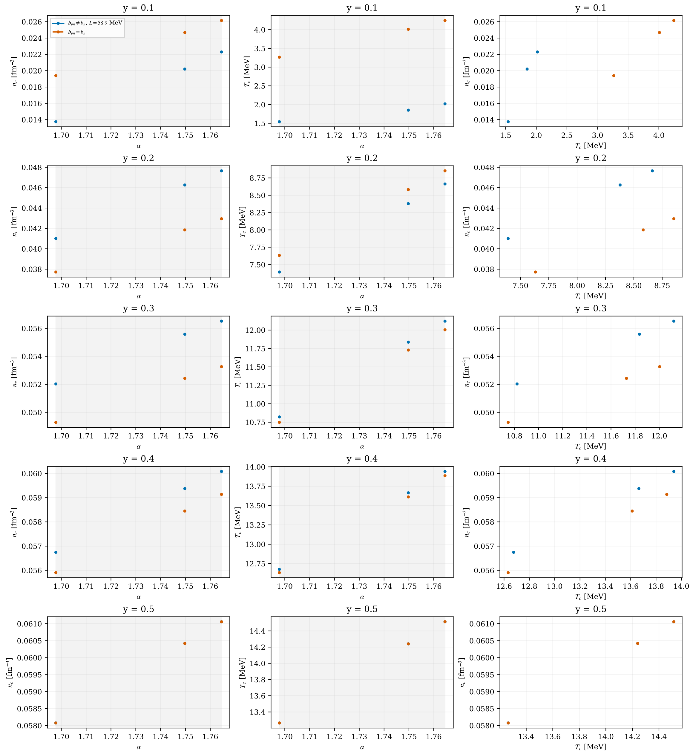
Dieterici-CS: fixed-composition critical points (30/140 solved) Gray: empirical parameter interval. Markers: solved points; gaps: missing/failed.
