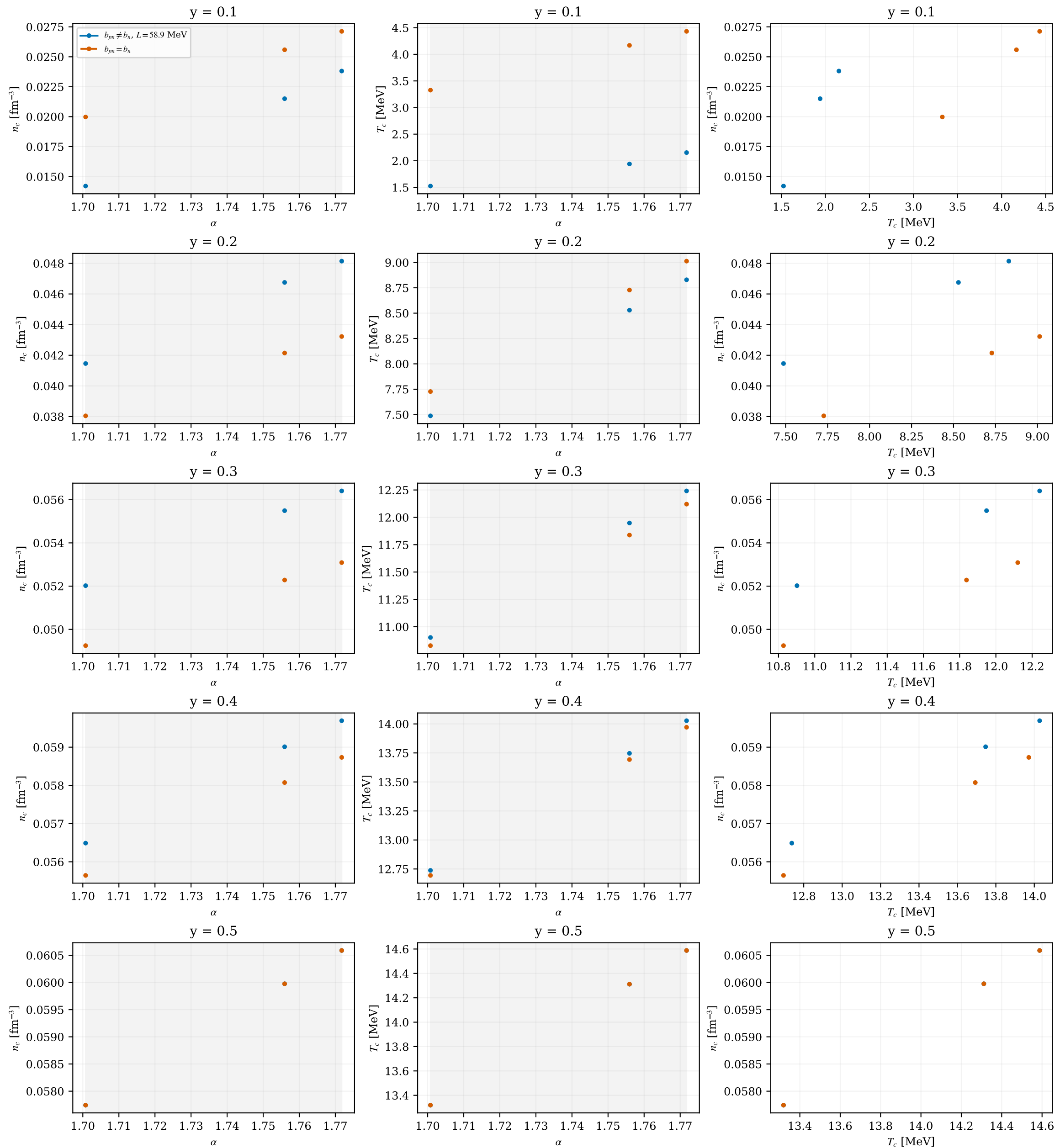
Dieterici-TVM: fixed-composition critical points (30/140 solved) Gray: empirical parameter interval. Markers: solved points; gaps: missing/failed.
