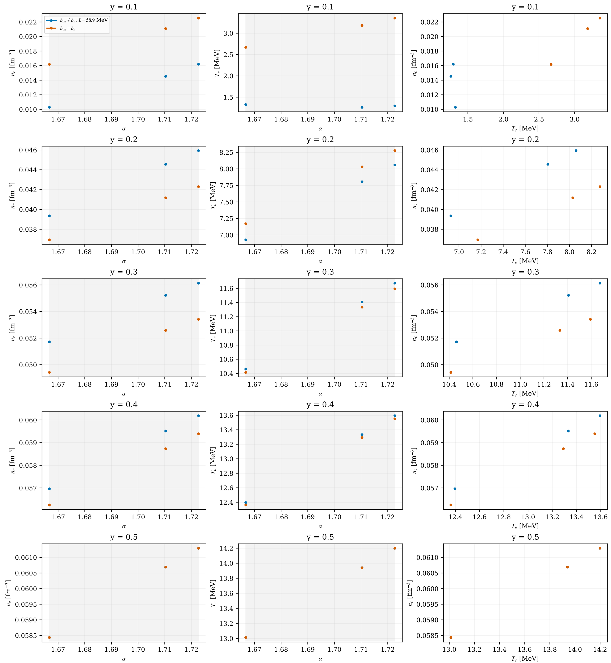
Dieterici-VDW: fixed-composition critical points (30/140 solved) Gray: empirical parameter interval. Markers: solved points; gaps: missing/failed.
