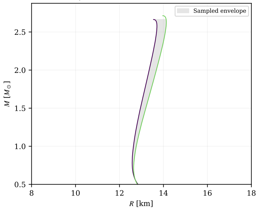
b_{pn} = b_n : 2/14 TOV
