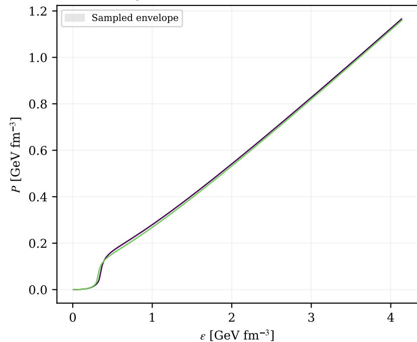
b_{pn} = b_n : 2/14 EoS
