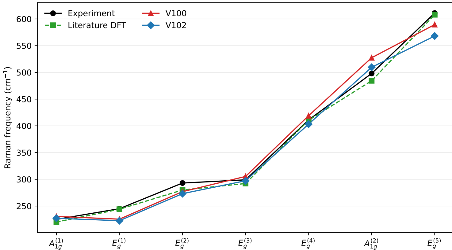
Bulk \alpha -Fe 2 O 3 : Raman-active \Gamma modes
