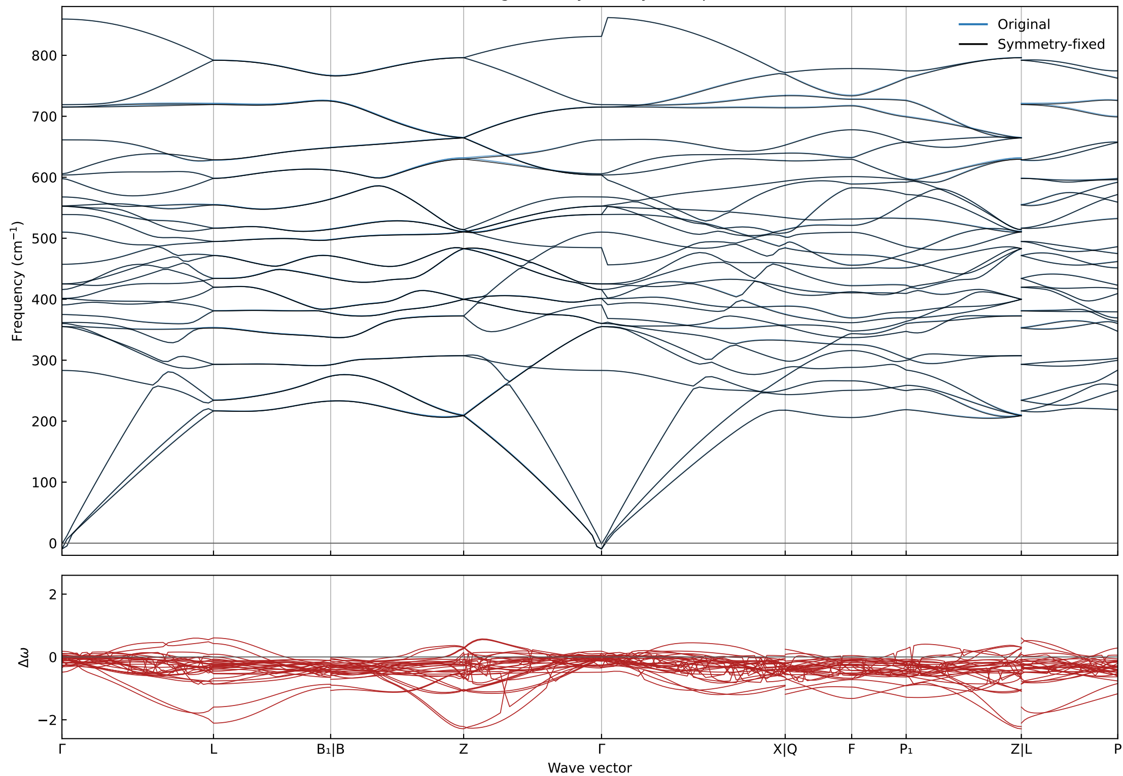
\alpha -Al 2 O 3 : original vs symmetry-fixed phonons
