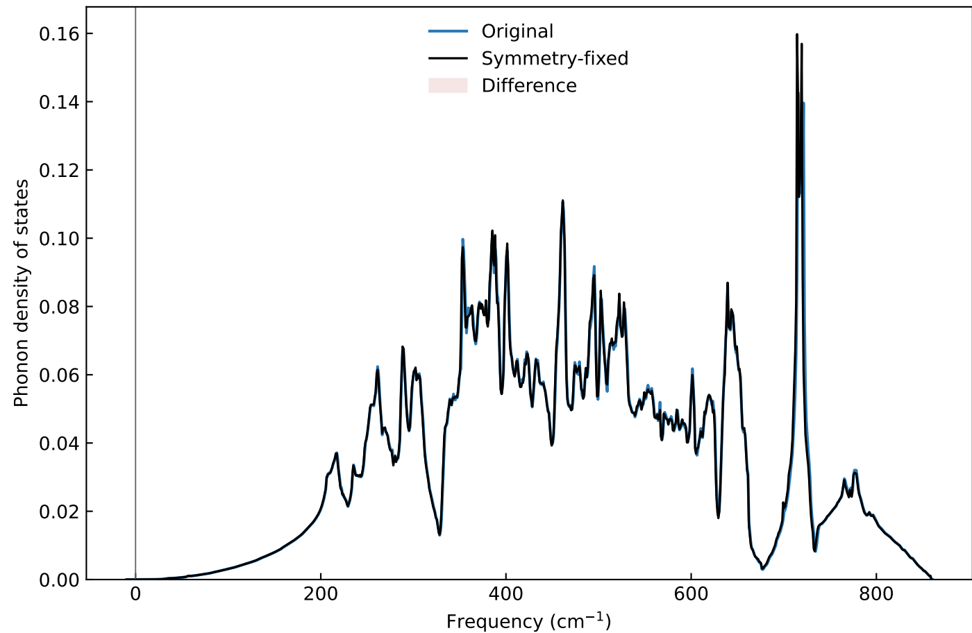
\alpha -Al 2 O 3 phonon DOS comparison
