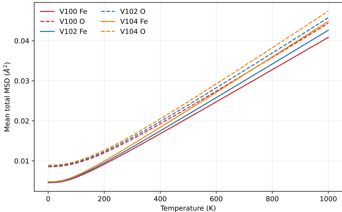
Harmonic atomic mean-square displacement
