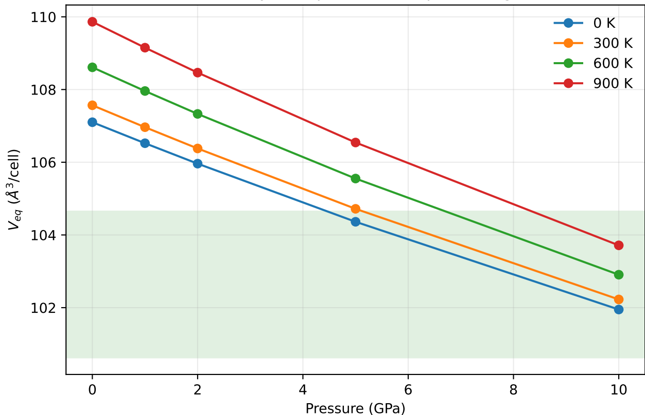
Preliminary QHA pressure-temperature grid
