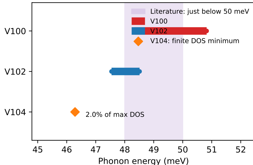
Low-DOS gap near 50 meV
