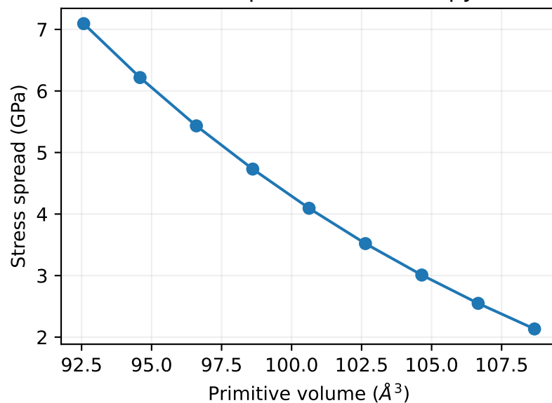
Fixed-shape stress anisotropy
