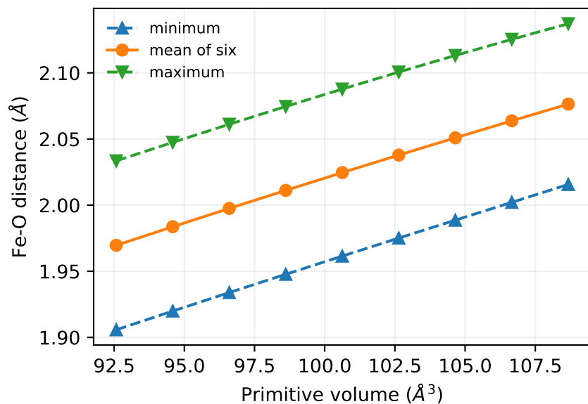
Relaxed FeO 6 coordination
