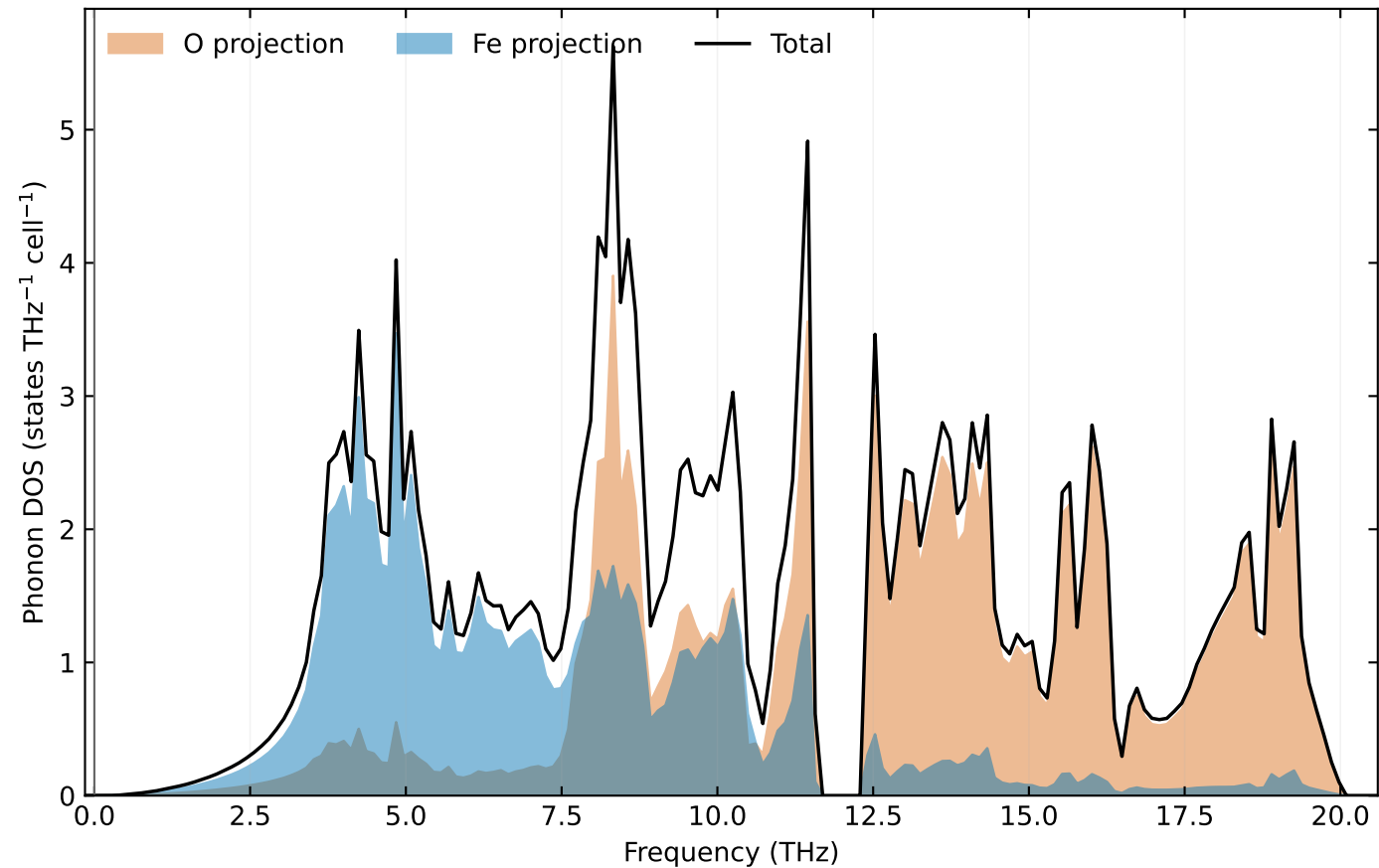
AFM \alpha -Fe 2 O 3 V100: species-projected phonon DOS
