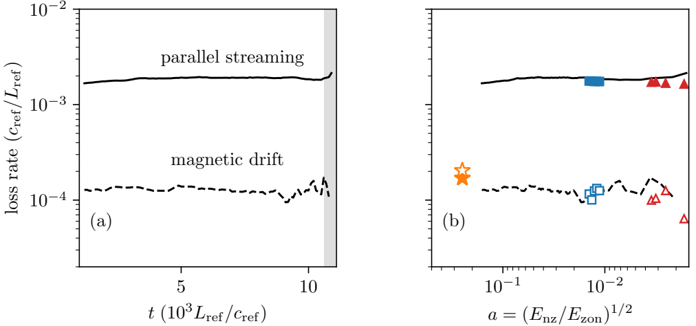
FIGURE 8. The channels through which the vortices lose electrostatic energy to entropy. (a) The rate of loss of E_{nz} , per unit E_{nz} , through the streaming of particles along the field line (solid) and through the magnetic drift (dashed), in sliding windows of about a hundred breathing periods of the original run; the grey band marks the collapse. (b) The same two rates against the amplitude measure a = (E_{nz}/E_{zon})^{1/2} , which decreases to the right, for the original run (lines) and the \epsilon = 0.3 (squares) and \epsilon = 0.03 (triangles) restarts, with filled symbols for the streaming and open ones for the drift, and for the production run of Kennedy & Plunk (2026b), whose box is four times larger in each perpendicular direction (stars). The loss is carried by the streaming of particles along the field line, at a rate that does not depend on the amplitude of the vortices and is smaller in the larger box.
