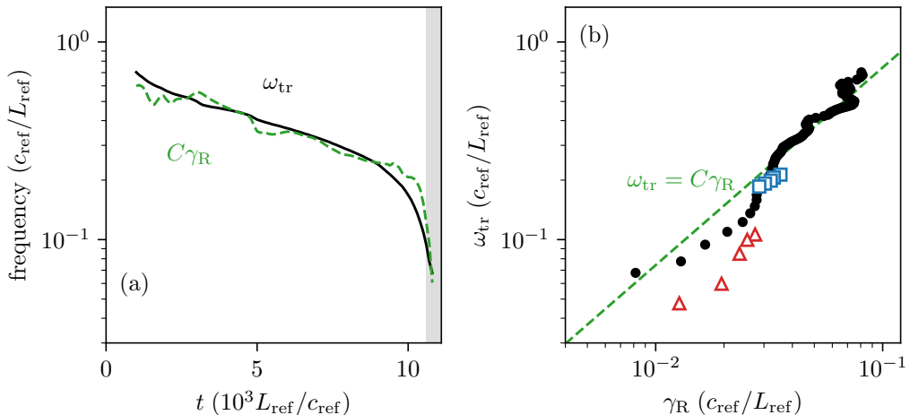
FIGURE 6. The saturation law (3.7). (a) The trapping frequency \omega_{\text{tr}} of the vortices, from (3.6) at their critical layers (black), and the growth rate \gamma_{\text{R}} of the unstable Rayleigh mode of the measured jets, multiplied by the constant C (green dashed), both as means over about eighty breathing periods; C is the geometric mean of their ratio, and the grey band marks the collapse. (b) The same data, \omega_{\text{tr}} against \gamma_{\text{R}} (black dots), with the line \omega_{\text{tr}} = C\gamma_{\text{R}} , and the \epsilon = 0.3 (blue squares) and \epsilon = 0.03 (red triangles) restarts, with \gamma_{\text{R}} computed on their own jets. The growth rate is that of the inviscid problem, converged in radial resolution. The trapping frequency of the vortices and the growth rate of the instability of their jets decay together, in a fixed ratio.
