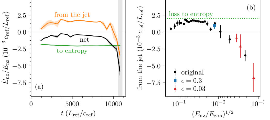
FIGURE 7. The budget (3.9) of the electrostatic energy of the vortices, averaged over the breathing. (a) The rates of change of E_{nz} , per unit E_{nz} , due to the nonlinear exchange with the zonal flow, \mathcal{T}/E_{nz} (orange), due to the linear terms, which convert electrostatic energy into entropy, -\mathcal{L}/E_{nz} (green), and their sum (black); the bands are standard errors over consecutive windows, and the grey band marks the collapse. (b) The exchange \mathcal{T}/E_{nz} against the amplitude measure a = (E_{nz}/E_{zon})^{1/2} , which decreases to the right, for the original run (black dots) and for the \epsilon = 0.3 (blue square) and \epsilon = 0.03 (red triangles) restarts; the dotted line is the magnitude of the loss. The vortices lose electrostatic energy to entropy at a steady rate that does not depend on their amplitude; the jets replace most of it while they are unstable, and the decay accelerates because that supply fades and finally reverses.
