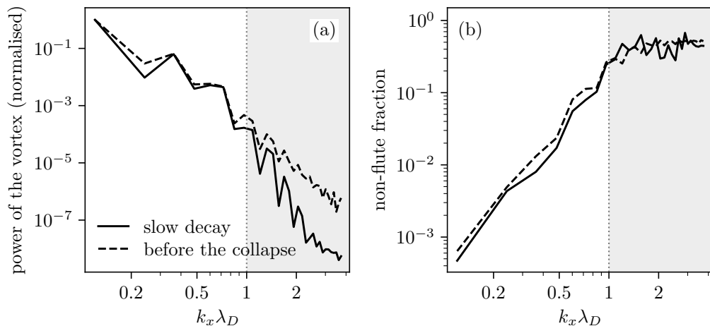
FIGURE 9. Flute character of the vortices, scale by scale. (a) The power of the k_y = 1 potential, summed along the field line and averaged over all output times in the slow phase of the decay (solid line) and in the approach to the collapse (dashed line), against the radial wavenumber k_x \lambda_D , each normalised to its maximum. (b) The fraction of that power that is not flute-like, i.e., the power of the departure of the potential from its mean along the field line divided by the total, for the same two intervals. The vertical dotted line marks k_x \lambda_D = 1 , and scales smaller than the Debye length are shaded. The vortices are flute-like at the scale of the box and lose their flute character at the Debye scale.
