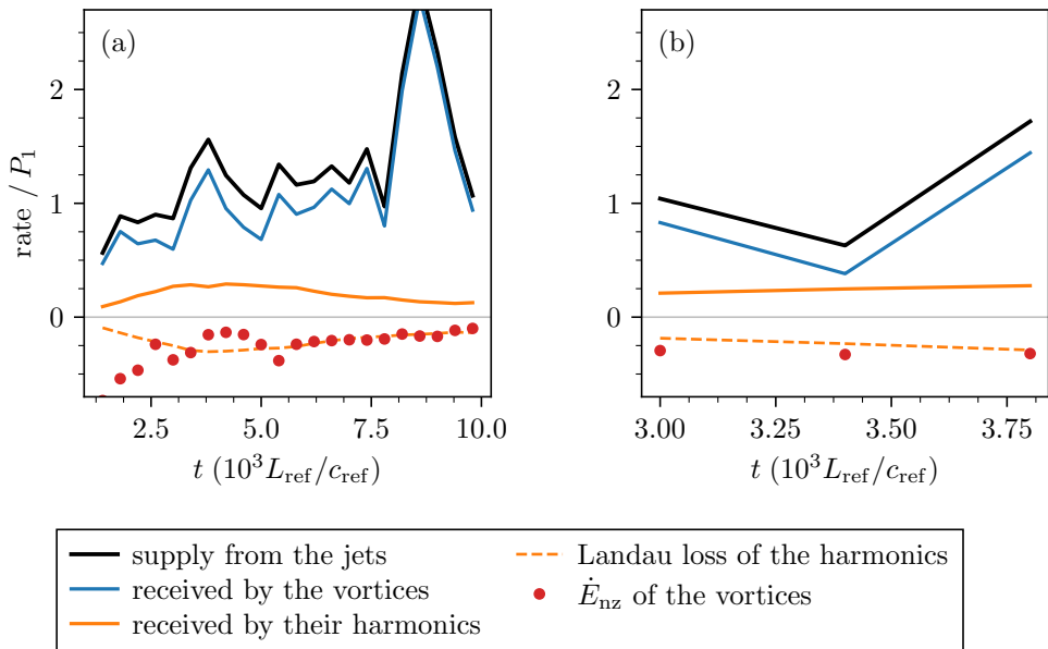
FIGURE 14. Where the energy goes, from the energy budget of the simulation resolved by binormal wavenumber, in the runs without radial hyperdiffusion: (a) at the resolution of the reference run, (b) at doubled radial resolution. All rates are divided by the Landau loss rate P_1 of the vortices: the nonlinear supply from the jets (black), the part of it received by the vortices (blue) and by their harmonics (orange), the Landau loss of the harmonics (orange dashed), and the rate of change of the energy of the vortices (red dots), in windows of eight hundred time units. The jets supply about the Landau loss of the vortices; the vortices pass a fifth of what they receive to their harmonics, which lose it at once, and drain by the remainder.
