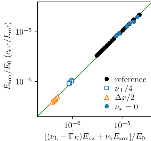
FIGURE 15. How the jets pay. The rate -\dot{E}_{zon} at which the jets lose electrostatic energy, against the part of the kinetic loss of the vortices that they do not drain, (\nu_L - \Gamma_E)E_{nz} , plus the radial hyperdiffusion of the jets, \nu_h E_{zon} , in windows of about four hundred time units, for the reference run, the restarts with the perpendicular hyperdiffusion divided by four and with doubled radial resolution, and the run without radial hyperdiffusion; the line is equality and there is no adjustable constant. The jets pay for the part of the loss that the vortices do not drain.
