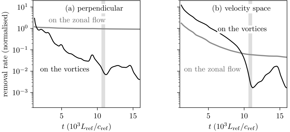
FIGURE 10. Where the free energy is removed. The rate of removal by (a) the perpendicular and (b) the velocity-space hyperdiffusion, each split into the part that acts on the zonal ( k_y = 0 ; grey) and on the non-zonal ( k_y \geq 1 ; black) part of the distribution, in sliding windows of about a hundred breathing periods, in units of the perpendicular removal from the zonal part in the slow phase of the decay; the parallel sink is negligible and is not shown. The grey band marks the collapse. The perpendicular sink acts on the zonal flow, whether or not there are vortices; the velocity-space sink acts mainly on the vortices, and falls away with them.
