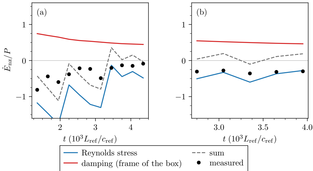
FIGURE 13. The energy of the vortices as the difference of two exchanges with the jets, in the runs without radial hyperdiffusion: (a) at the resolution of the reference run, (b) at doubled radial resolution. The rate at which the vortices gain energy through the Reynolds stress of their field-line-averaged potential (blue) and through their Landau damping in the frame of the box (red), the sum of the two (grey dashed) and the measured rate of change of their energy (dots), all divided by the absorbed power P , in windows of three hundred time units. The two exchanges are each of the order of the absorbed power and of opposite sign; the vortices drain by their small difference.
