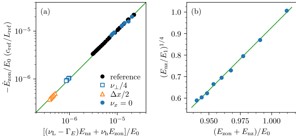
FIGURE 15. How the jets pay. (a) The rate -\dot{E}_{\text{zon}} at which the jets lose electrostatic energy, against the part of the kinetic loss of the vortices that they do not drain, (\nu_L - \Gamma_E)E_{\text{nz}} , plus the radial hyperdiffusion of the jets, \nu_h E_{\text{zon}} , in windows of about four hundred time units, for the reference run, the restarts with the perpendicular hyperdiffusion divided by four and with doubled radial resolution, and the run without radial hyperdiffusion; the line is equality and there is no adjustable constant. (b) In the run without radial hyperdiffusion, E_{\text{nz}}^{1/4} against the total electrostatic energy. The jets pay for the part of the loss that the vortices do not drain.
