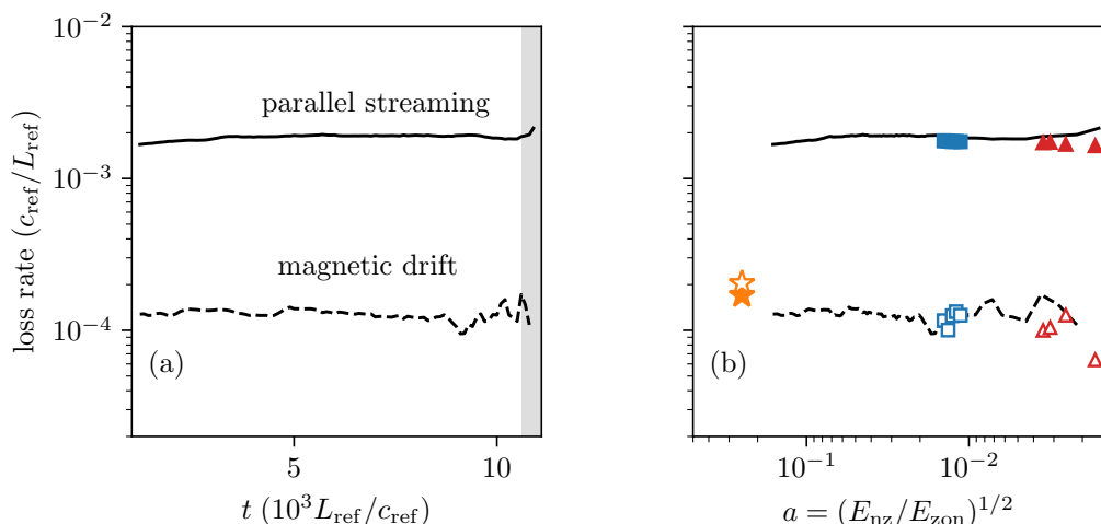
FIGURE 9. The channels through which the vortices lose electrostatic energy to entropy. (a) The rate of loss of E_{nz} , per unit E_{nz} , through the streaming of particles along the field line (solid) and through the magnetic drift (dashed), in sliding windows of about a hundred breathing periods of the original run; the grey band marks the collapse. (b) The same two rates against the amplitude measure a = (E_{nz}/E_{zon})^{1/2} , which decreases to the right, for the original run (lines) and the \epsilon = 0.3 (squares) and \epsilon = 0.03 (triangles) restarts, with filled symbols for the streaming and open ones for the drift, and for the production run of Kennedy & Plunk (2026b), whose box is four times larger in each perpendicular direction (stars). The loss is carried by the streaming of particles along the field line, at a rate that does not depend on the amplitude of the vortices and is smaller in the larger box.
