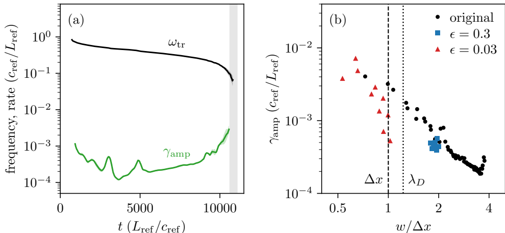
FIGURE 13. Time scales of the vortices and the approach to the collapse. (a) The trapping frequency \omega_{\text{tr}} of (3.6) at the critical layer (black) and the amplitude decay rate \gamma_{\text{amp}} = I_E/2 (green), each as the geometric mean of the two vortices on a band that spans them; \gamma_{\text{amp}} is from sliding fits of the logarithm of the energy of each vortex in windows of about a hundred breathing periods, and the grey band marks the collapse. (b) The decay rate of each vortex, from fits in windows half as long, against the half-width w of its cat's eye in units of the grid spacing, for the original run (black dots) and for the \epsilon = 0.3 (blue squares) and \epsilon = 0.03 (red triangles) restarts after their regrowth; the dashed and dotted vertical lines mark w = \Delta x and w = \lambda_D . The fluid in the cat's eyes turns over many times while the vortices decay, and the decay speeds up as the cat's eyes narrow towards one grid cell, which is also about one Debye length.
