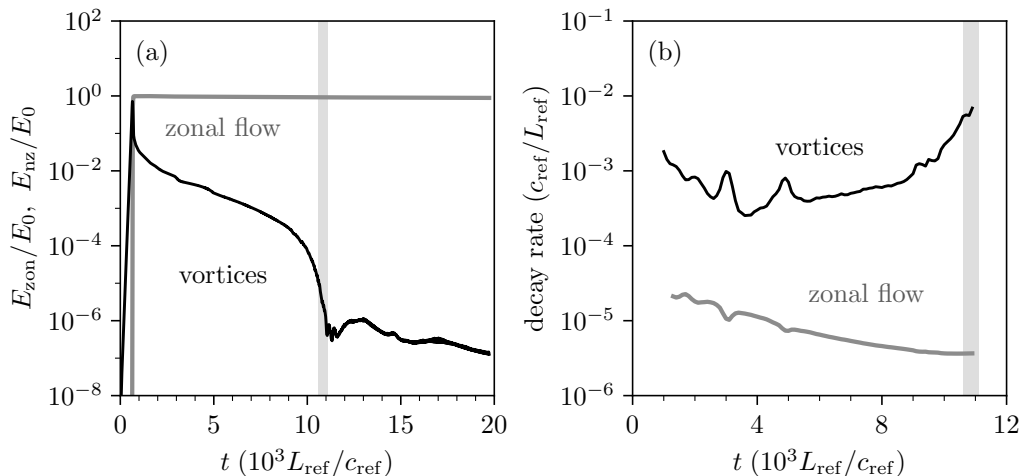
FIGURE 2. Electrostatic energy of the zonal flow and of the vortices in the reduced-box simulation. (a) The zonal energy E_{\text{zon}} (grey) and the non-zonal energy E_{\text{nz}} (black), as running means over about ten breathing periods, in units of E_0 , the largest value of E_{\text{zon}} . (b) The decay rates \Gamma_E = -d \ln E_{\text{nz}}/dt (black) and -d \ln E_{\text{zon}}/dt (grey), from least-squares fits of the logarithm of each energy in sliding windows of about a hundred breathing periods, from the end of the relaxation that follows the burst to the end of the collapse. The grey band marks the collapse in this and all subsequent figures. The vortices lose many decades of energy, ever faster and without a plateau, and then collapse, while the zonal flow barely changes.
