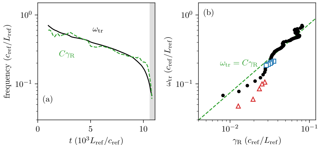
FIGURE 7. The saturation law (3.7). (a) The trapping frequency \omega_{tr} of the vortices, from (3.6) at their critical layers (black), and the growth rate \gamma_R of the unstable Rayleigh mode of the measured jets, multiplied by the constant C (green dashed), both as means over about eighty breathing periods; C is the geometric mean of their ratio, and the grey band marks the collapse. (b) The same data, \omega_{tr} against \gamma_R (black dots), with the line \omega_{tr} = C\gamma_R , and the \epsilon = 0.3 (blue squares) and \epsilon = 0.03 (red triangles) restarts, with \gamma_R computed on their own jets. The growth rate is that of the inviscid problem, converged in radial resolution. The trapping frequency of the vortices and the growth rate of the instability of their jets decay together, in a fixed ratio.
