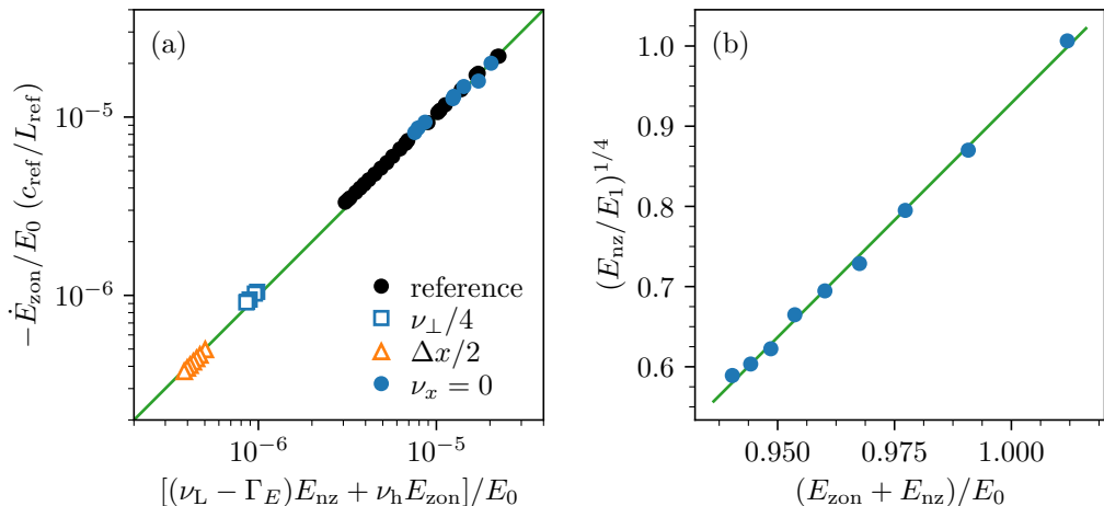
FIGURE 17. How the jets pay. (a) The rate -\dot{E}_{\text{zon}} at which the jets lose electrostatic energy, against the part of the kinetic loss of the vortices that they do not drain, (\nu_L - \Gamma_E)E_{\text{nz}} , plus the radial hyperdiffusion of the jets, \nu_h E_{\text{zon}} , in windows of about four hundred time units, for the reference run, the restarts with the perpendicular hyperdiffusion divided by four and with doubled radial resolution, and the run without radial hyperdiffusion; the line is equality and there is no adjustable constant. (b) In the run without radial hyperdiffusion, E_{\text{nz}}^{1/4} against the total electrostatic energy. The jets pay for the part of the loss that the vortices do not drain.
