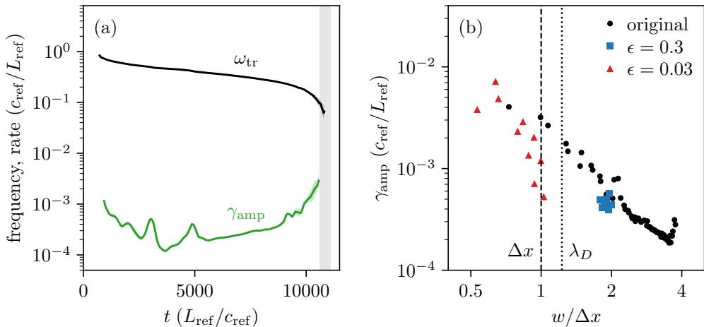
FIGURE 14. Time scales of the vortices and the approach to the collapse. (a) The trapping frequency \omega_{\text{tr}} of (3.6) at the critical layer (black) and the amplitude decay rate \gamma_{\text{amp}} = I_E/2 (green), each as the geometric mean of the two vortices on a band that spans them; \gamma_{\text{amp}} is from sliding fits of the logarithm of the energy of each vortex in windows of about a hundred breathing periods, and the grey band marks the collapse. (b) The decay rate of each vortex, from fits in windows half as long, against the half-width w of its cat's eye in units of the grid spacing, for the original run (black dots) and for the \epsilon = 0.3 (blue squares) and \epsilon = 0.03 (red triangles) restarts after their regrowth; the dashed and dotted vertical lines mark w = \Delta x and w = \lambda_D . The fluid in the cat's eyes turns over many times while the vortices decay, and the decay speeds up as the cat's eyes narrow towards one grid cell, which is also about one Debye length.
