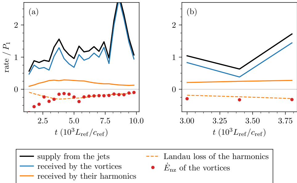
FIGURE 16. Where the energy goes, from the energy budget of the simulation resolved by binormal wavenumber, in the runs without radial hyperdiffusion: (a) at the resolution of the reference run, (b) at doubled radial resolution. All rates are divided by the Landau loss rate P_1 of the vortices: the nonlinear supply from the jets (black), the part of it received by the vortices (blue) and by their harmonics (orange), the Landau loss of the harmonics (orange dashed), and the rate of change of the energy of the vortices (red dots), in windows of eight hundred time units. The jets supply about the Landau loss of the vortices; the vortices pass a fifth of what they receive to their harmonics, which lose it at once, and drain by the remainder.
