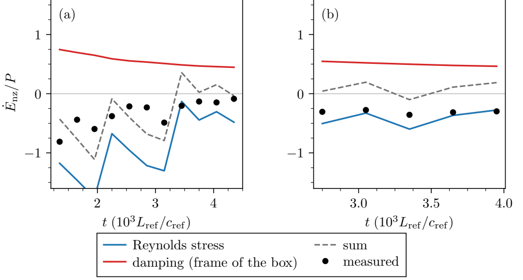
FIGURE 15. The energy of the vortices as the difference of two exchanges with the jets, in the runs without radial hyperdiffusion: (a) at the resolution of the reference run, (b) at doubled radial resolution. The rate at which the vortices gain energy through the Reynolds stress of their field-line-averaged potential (blue) and through their Landau damping in the frame of the box (red), the sum of the two (grey dashed) and the measured rate of change of their energy (dots), all divided by the absorbed power P , in windows of three hundred time units. The two exchanges are each of the order of the absorbed power and of opposite sign; the vortices drain by their small difference.
