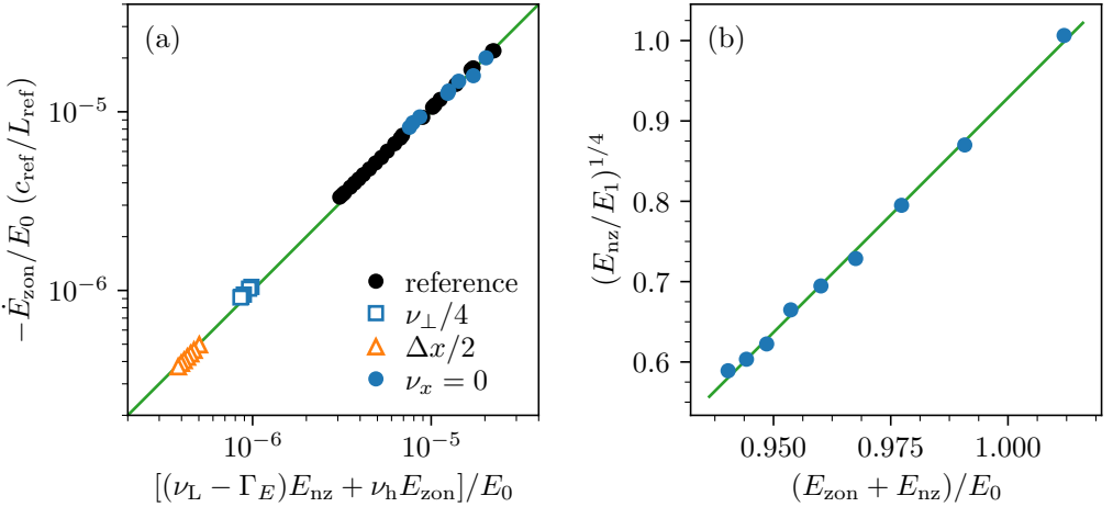
FIGURE 16. How the jets pay. (a) The rate -\dot{E}_{zon} at which the jets lose electrostatic energy, against the part of the kinetic loss of the vortices that they do not drain, (\nu_L - \Gamma_E)E_{nz} , plus the radial hyperdiffusion of the jets, \nu_h E_{zon} , in windows of about four hundred time units, for the reference run, the restarts with the perpendicular hyperdiffusion divided by four and with doubled radial resolution, and the run without radial hyperdiffusion; the line is equality and there is no adjustable constant. (b) In the run without radial hyperdiffusion, E_{nz}^{1/4} against the total electrostatic energy. The jets pay for the part of the loss that the vortices do not drain.
