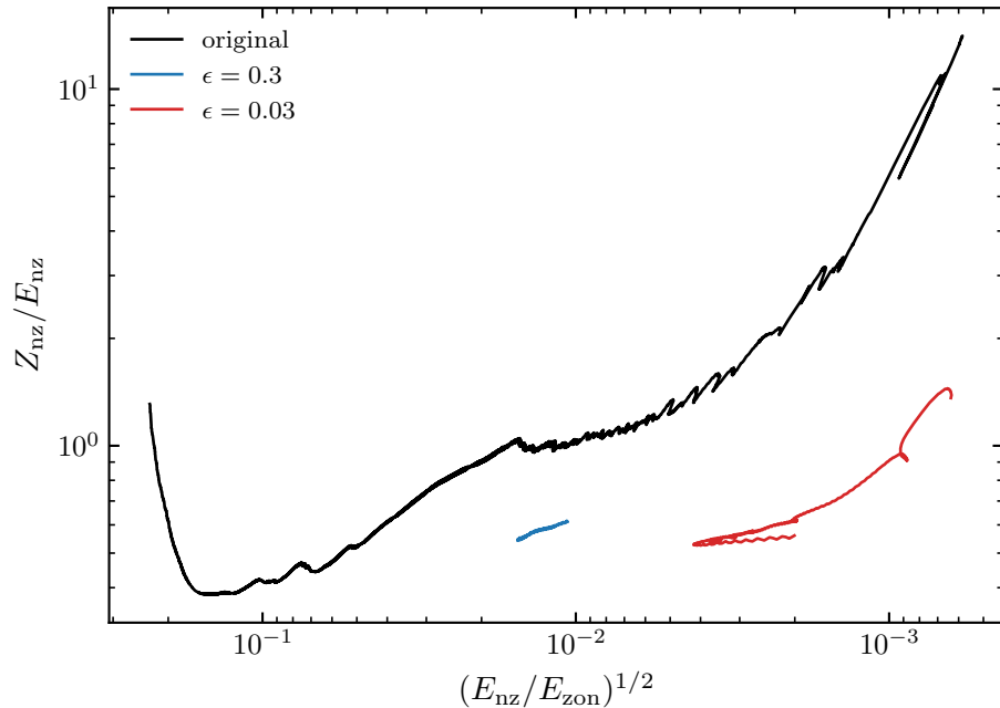
(b) entropy-to-energy ratio against amplitude
