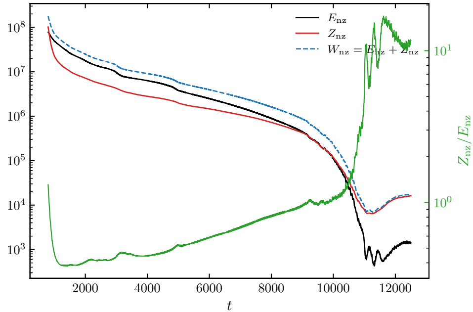
(a) original run (37-t.u. running means)
