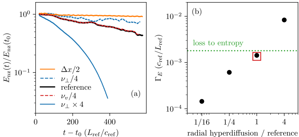
FIGURE 13. The sink tests: restarts of the reference run from one state in the accelerating phase of its decay, at time t_0 , each with one sink changed. (a) The non-zonal electrostatic energy, as running means over about ten breathing periods, for the reference run (black), for the velocity-space hyperdiffusion divided by four (red dashed, on top of the black), for the perpendicular hyperdiffusion multiplied by four (blue solid) and divided by four (blue dashed), and for the radial resolution doubled, which divides the radial hyperdiffusion at a given wavenumber by sixteen (orange). (b) The mean decay rate \Gamma_E over the interval of (a) against the strength of the radial hyperdiffusion relative to the reference run (black dots; the open red square is the run with the velocity-space hyperdiffusion divided by four), and the loss rate \mathcal{L}/E_{nz} to entropy, which is the same in all the runs (green dotted). The decay of the vortices follows the perpendicular sink, not the velocity-space one, and where the perpendicular sink is weak the vortices persist although they are Landau damped.
