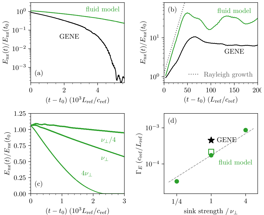
FIGURE 12. The two-dimensional fluid model against the kinetic simulation. (a) The non-zonal energy of the simulation (black) and of the fluid model started from its potential at the time t_0 of the amplitude tests (green). (b) The same for the restart with the vortices reduced by \epsilon = 0.03 , with growth at the Rayleigh rate (dotted). (c) The fluid model with its perpendicular sink multiplied by four, unchanged, and divided by four. (d) The decay rate of the fluid model against the strength of its sink (circles; the square is the same model at higher radial resolution), a linear dependence (dashed) and the simulation (star). All curves are running means over ten breathing periods [two in (b)]. A fluid with the perpendicular sink of the simulation reproduces the vortices, their regrowth and a part of their decay; the rest of the damping is kinetic.
