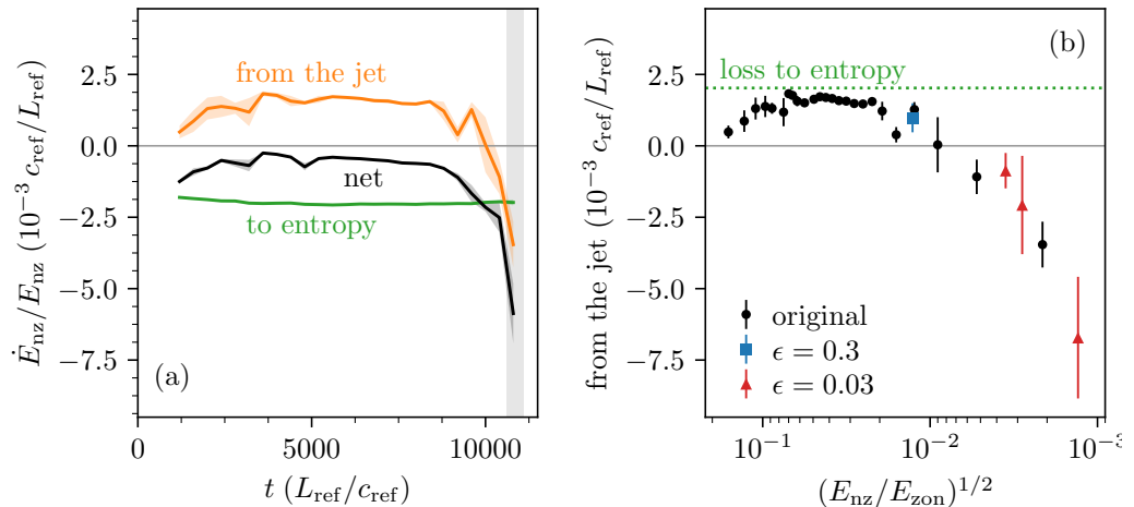
FIGURE 8. The budget (3.10) of the electrostatic energy of the vortices, averaged over the breathing. (a) The rates of change of E_{nz} , per unit E_{nz} , due to the nonlinear exchange with the zonal flow, \mathcal{T}/E_{nz} (orange), due to the linear terms, which convert electrostatic energy into entropy, -\mathcal{L}/E_{nz} (green), and their sum (black); the bands are standard errors over consecutive windows, and the grey band marks the collapse. (b) The exchange \mathcal{T}/E_{nz} against the amplitude measure a = (E_{nz}/E_{zon})^{1/2} , which decreases to the right, for the original run (black dots) and for the \epsilon = 0.3 (blue square) and \epsilon = 0.03 (red triangles) restarts; the dotted line is the magnitude of the loss. The vortices lose electrostatic energy to entropy at a steady rate that does not depend on their amplitude; the jets replace most of it while they are unstable, and the decay accelerates because that supply fades and finally reverses.
