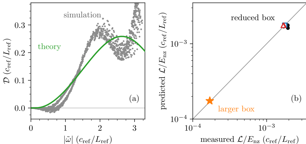
FIGURE 10. Landau damping of the non-flute part of the vortices: theory against simulation. (a) The dissipation function \mathcal{D} of (C 13) against the local Doppler-shifted frequency |\tilde{\omega}| : the solution of (C 11) in the magnetic geometry of the flux tube (green line), and its measured counterpart, viz., the part of the non-flute potential that lags behind its forcing, at every radius where either vortex is appreciable and at many times through the decay of the reduced-box run (grey dots). (b) The loss rate \mathcal{L}/E_{nz} predicted by (3.9) from the flute-like part of the vortices and the jets, against the rate measured by the energy diagnostics of the code in the channel of parallel streaming, for the reduced-box run through its decay (black dots), its \epsilon = 0.3 (blue squares) and \epsilon = 0.03 (red triangles) restarts, and the production run of Kennedy & Plunk (2026b), whose box is four times larger in each perpendicular direction (orange star); the line is equality. The vortices lose their energy by Landau damping of their non-flute part, at the rate that the theory gives, with no adjustable parameter, in every run.
