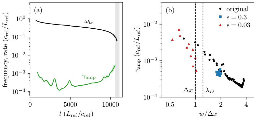
FIGURE 14. Time scales of the vortices and the approach to the collapse. (a) The trapping frequency \omega_{tr} of (3.6) at the critical layer (black) and the amplitude decay rate \gamma_{amp} = I_E/2 (green), each as the geometric mean of the two vortices on a band that spans them; \gamma_{amp} is from sliding fits of the logarithm of the energy of each vortex in windows of about a hundred breathing periods, and the grey band marks the collapse. (b) The decay rate of each vortex, from fits in windows half as long, against the half-width w of its cat's eye in units of the grid spacing, for the original run (black dots) and for the \epsilon = 0.3 (blue squares) and \epsilon = 0.03 (red triangles) restarts after their regrowth; the dashed and dotted vertical lines mark w = \Delta x and w = \lambda_D . The fluid in the cat's eyes turns over many times while the vortices decay, and the decay speeds up as the cat's eyes narrow towards one grid cell, which is also about one Debye length.
