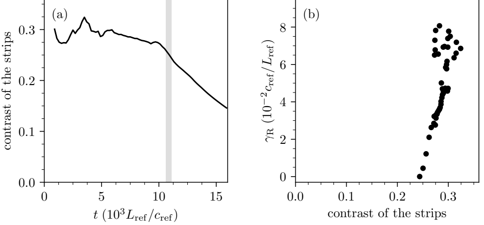
FIGURE 6. The corrugation of the jets. (a) The contrast of the vorticity strips, viz., the mean of |U'| on the two strips of a shear layer less its value midway between them, divided by the largest |U'| and averaged over the two shear layers, for the zonal flow averaged over about sixteen breathing periods; the grey band marks the collapse. (b) The growth rate \gamma_R of the unstable Rayleigh mode against the contrast, up to the collapse. The corrugation hardly changes while the vortices are present and decays once they have gone, and the jets are only just unstable: the growth rate vanishes at a finite contrast.
