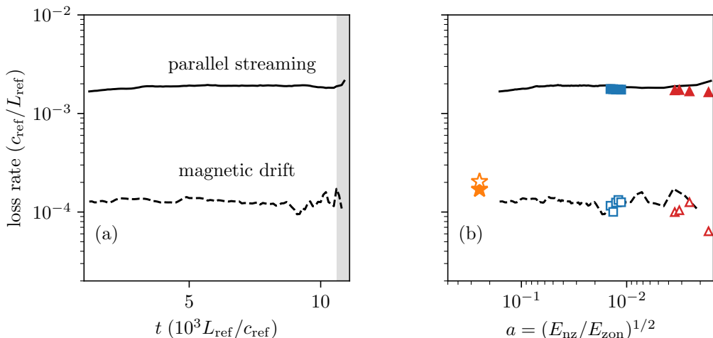
FIGURE 9. The channels through which the vortices lose electrostatic energy to entropy. (a) The rate of loss of E_{\text{nz}} , per unit E_{\text{nz}} , through the streaming of particles along the field line (solid) and through the magnetic drift (dashed), in sliding windows of about a hundred breathing periods of the original run; the grey band marks the collapse. (b) The same two rates against the amplitude measure a = (E_{\text{nz}}/E_{\text{zon}})^{1/2} , which decreases to the right, for the original run (lines) and the \epsilon = 0.3 (squares) and \epsilon = 0.03 (triangles) restarts, with filled symbols for the streaming and open ones for the drift, and for the production run of Kennedy & Plunk (2026b), whose box is four times larger in each perpendicular direction (stars). The loss is carried by the streaming of particles along the field line, at a rate that does not depend on the amplitude of the vortices and is smaller in the larger box.
