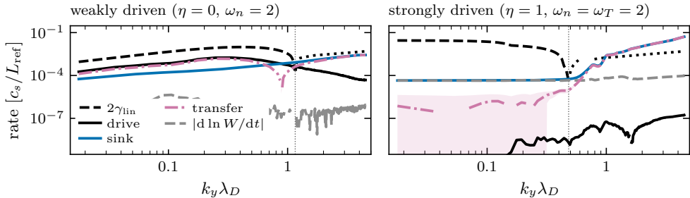
FIGURE 12. Every term of the per- k_y free-energy budget (4.9) as a rate, each channel divided by the free energy of the same k_y and time-averaged. Left-hand side : the weakly driven baseline, over the arrested floor. Right-hand side : above the fluid threshold, over the drainage. Each panel carries the drive, the sink, the transfer between modes and the rate at which the mode's own free energy changes, against the linear reference 2\gamma_{\text{lin}}(k_y) , dashed where the linear mode grows and dotted where it is damped. The transfer is the term that closes the budget; where it does not exceed the spread of three estimators of the store's decay it is drawn dotted, with that spread shaded. Curves carry magnitudes and break where a term changes sign; the transfer is negative at long wavelength and positive at short, and the store falls at \eta = 1 where at \eta = 0 it is steady. The vertical dotted line marks where the linear growth rate changes sign. Both axes logarithmic.
