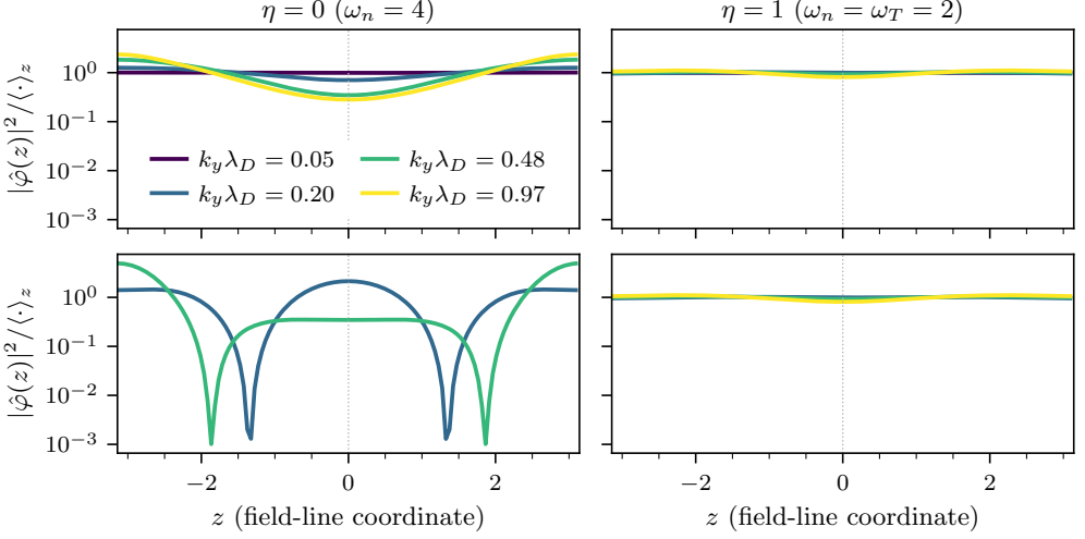
FIGURE 20. Parallel structure |\hat{\varphi}(z)|^2 (normalised to its z -mean, log scale) of the linear eigenmodes at c_{\text{surf}} = 1.2 , one curve per k_y (coloured by k_y ). Only unstable modes are drawn. Left column: \eta = 0 , \omega_n = 4 . Right column: \eta = 1 , \omega_n = \omega_T = 2 . Top row: dominant eigenmode. Bottom row: the sub-dominant unstable eigenmode where one exists, which is a second purely growing root at \eta = 0 and the complex-conjugate partner of the dominant mode beyond the branch collision at \eta = 1 . z = 0 is the field minimum (apex), z = \pm\pi the field maxima.
