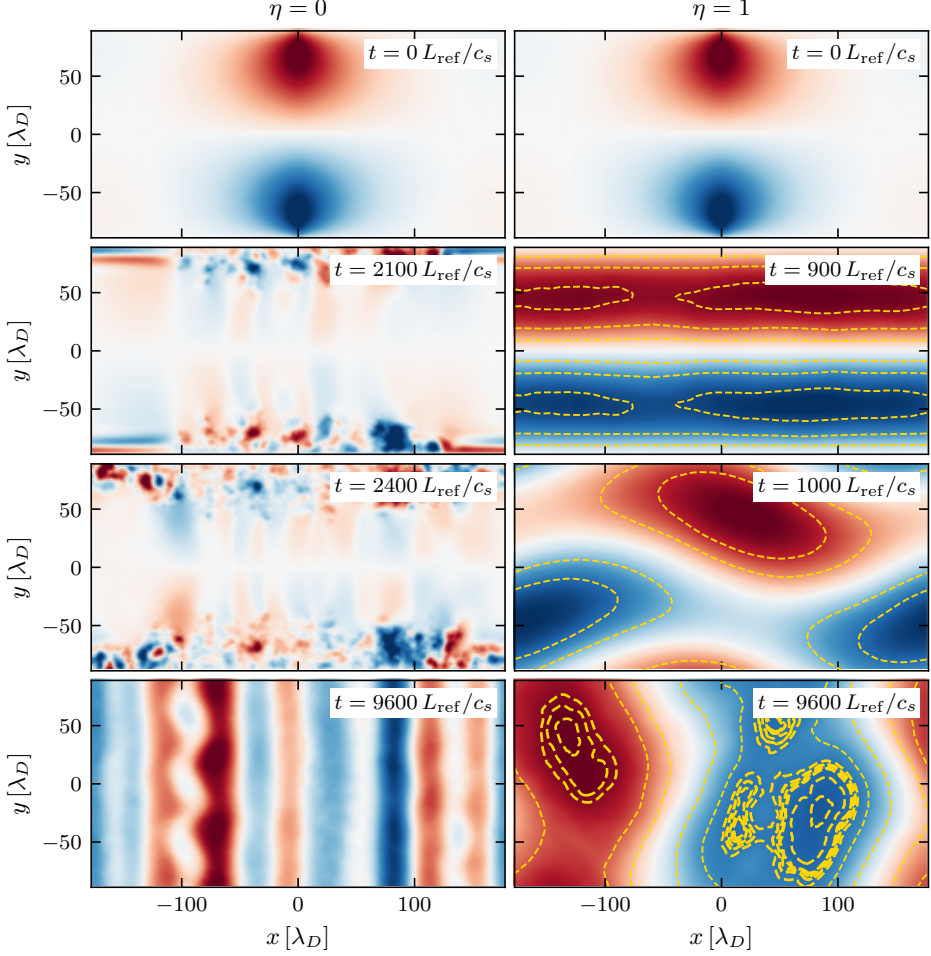
FIGURE 15. Formation of the dipole state at the z = 0 equator: potential \phi(x, y) at c_{\text{surf}} = 1.10 in the radially elongated box of appendix F ( 2:1 in x:y ). Left column: \eta = 0 , \omega_n = 2 . Right column: \eta = 1 , \omega_n = \omega_T = 2 . Rows, top to bottom: close to the initial condition, formation of streamers, the secondary instability, the developed state. Colour scales saturate at the 99th percentile of each panel, and gold dashed contours on the \eta = 1 column mark fixed fractions of each panel's colour scale, as in Figure 9.
