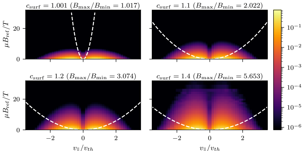
FIGURE 22. Velocity-space resolution check across the dipole c_{\text{surf}} scan: |\langle f \rangle|^2 of the dominant linear eigenmode, summed over z and species, on the (v_{||}, \mu) plane at fixed k_y \lambda_D = 0.068 for c_{\text{surf}} = 1.001, 1.10, 1.20, 1.40 (panels left to right, top to bottom, with the well depth B_{\text{max}}/B_{\text{min}} in each title), at \eta = 1, \omega_n = \omega_T = 2 , on the eigenvalue-scan velocity-space grid. White dashed: the trapped/passing boundary at the z = 0 slice.
