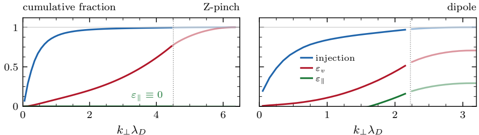
FIGURE 16. Cumulative k_\perp removal of the free energy by channel at the \eta = 0 , \omega_n = 2 drive: the velocity-space sink \varepsilon_v and the parallel sink \varepsilon_\parallel as fractions of the total removal, with the injection spectrum for reference. Left : Z-pinch, averaged over t = 20\,000 – 25\,000\,L_{\text{ref}}/c_s . Right : dipole at c_{\text{surf}} = 1.10 , averaged over t = 5600 – 8000\,L_{\text{ref}}/c_s . Complete k_\perp shells are drawn solid to the dotted line. Beyond it the rectangular box no longer contains every mode of a shell and the faded curves are only partial-shell estimates.
