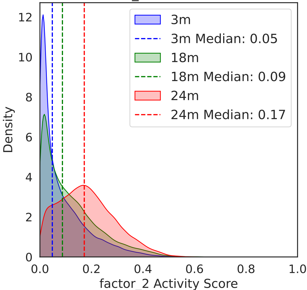
Factor factor_2 Distribution for None
