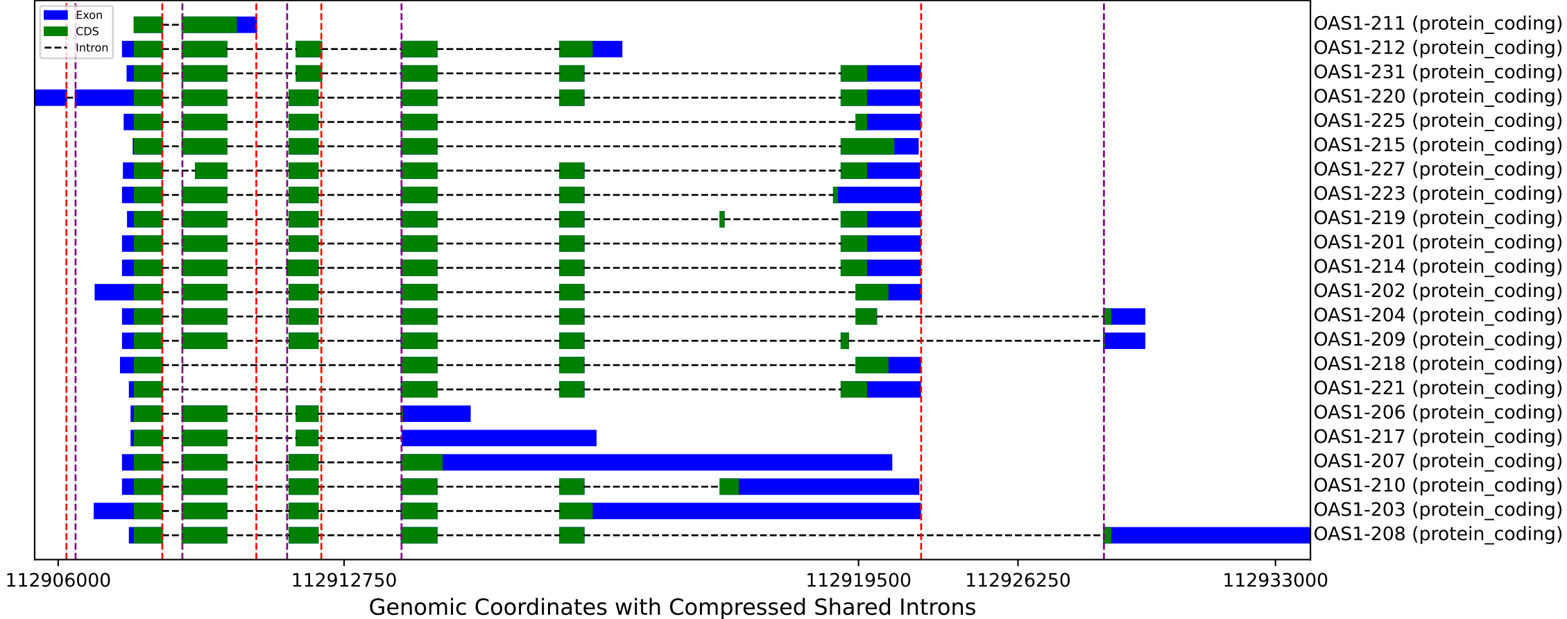
Isoforms (Exons and CDS) for Gene OAS1 (ID: ENSG00000089127.15, Strand: +)
