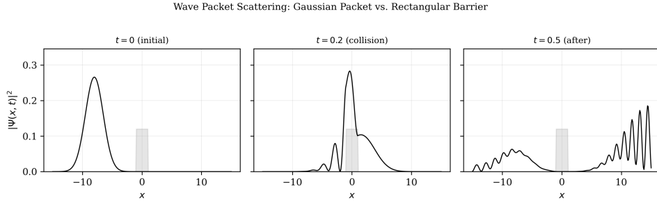
Figure 8: Temporal snapshots of probability density |\Psi(x, t)|^2 during wave packet collision with a rectangular barrier, illustrating spatial bifurcation into transmitted and reflected wave packets.
