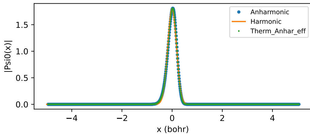
vib6 Wavefunction
