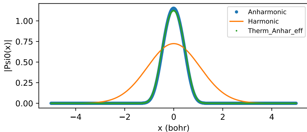
vib2 Wavefunction
