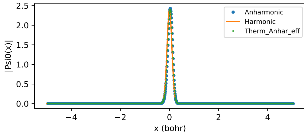
vib3 Wavefunction
