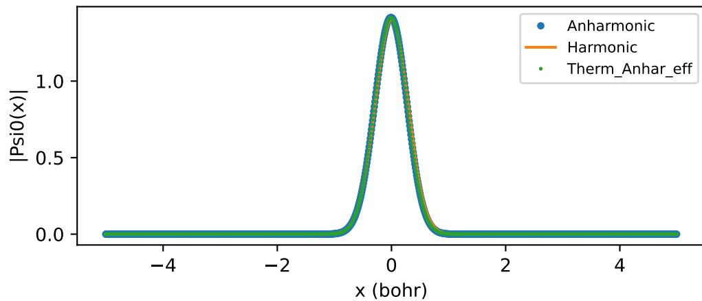
vib5 Wavefunction
