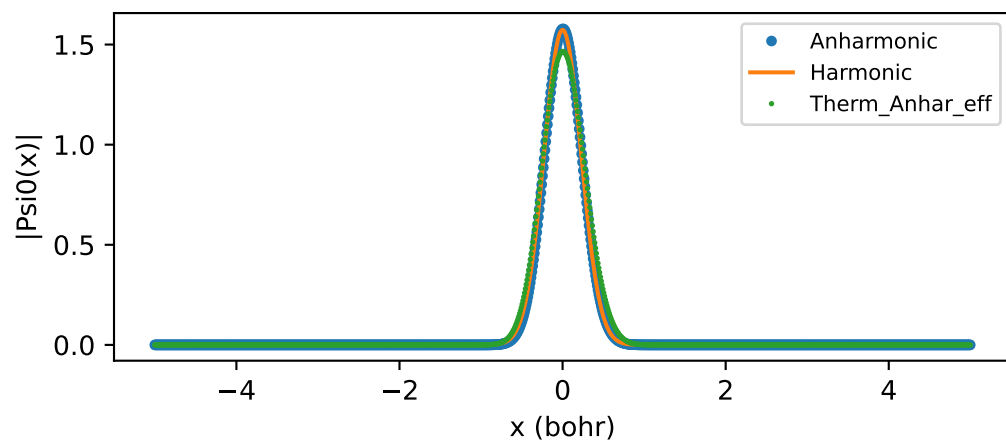
vib3 Wavefunction
