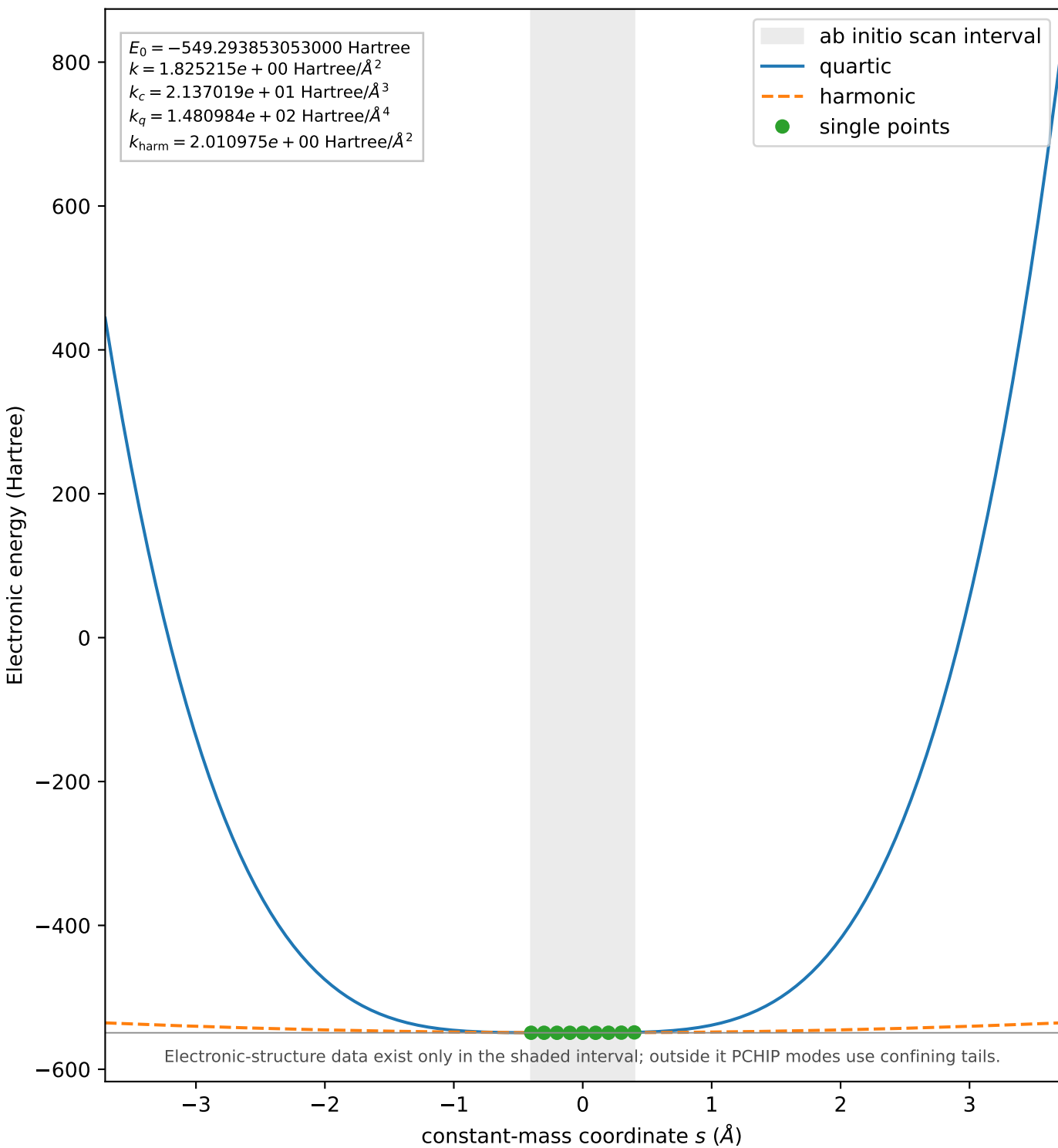
Mode 6: full potential diagnostic (−7 to +7 bohr)
