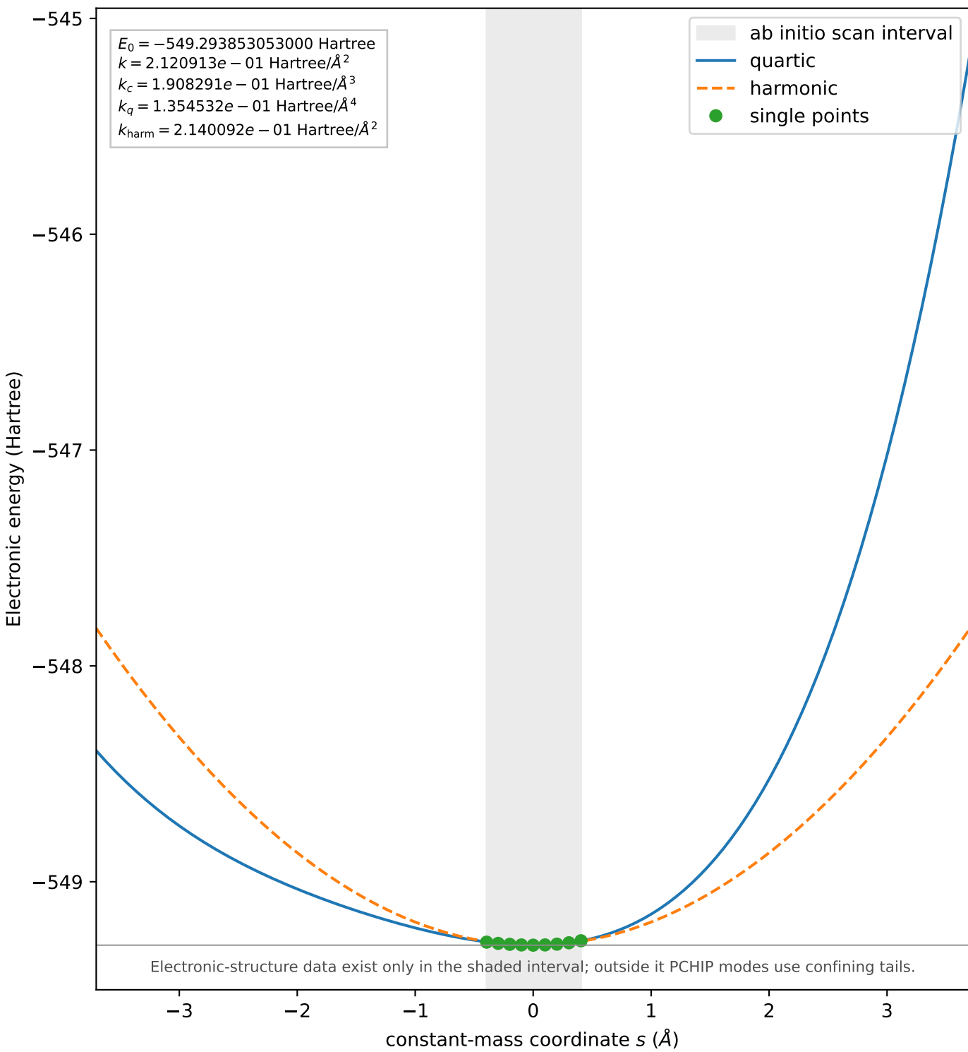
Mode 4: full potential diagnostic (−7 to +7 bohr)
