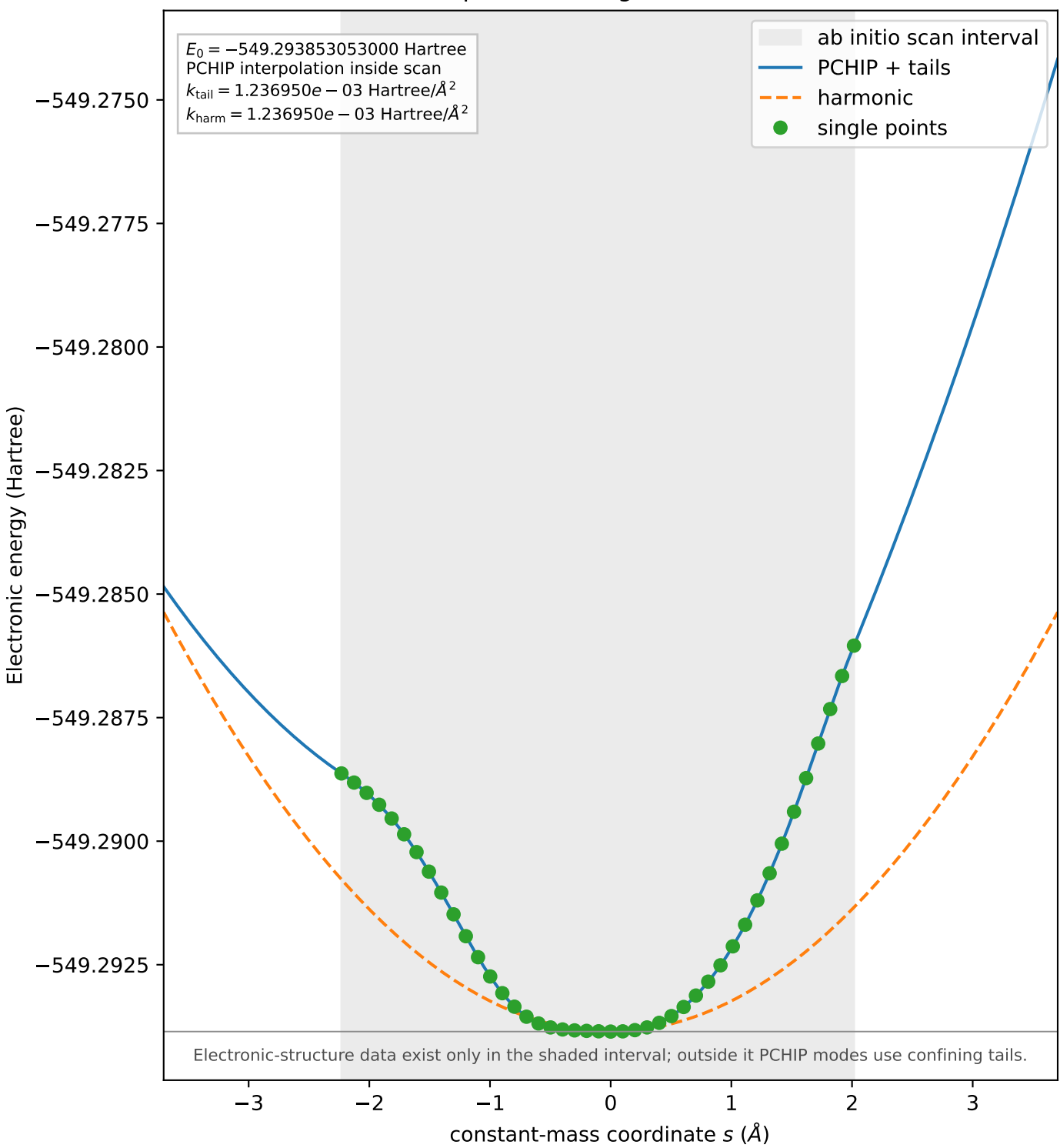
Mode 1: full potential diagnostic (−7 to +7 bohr)
