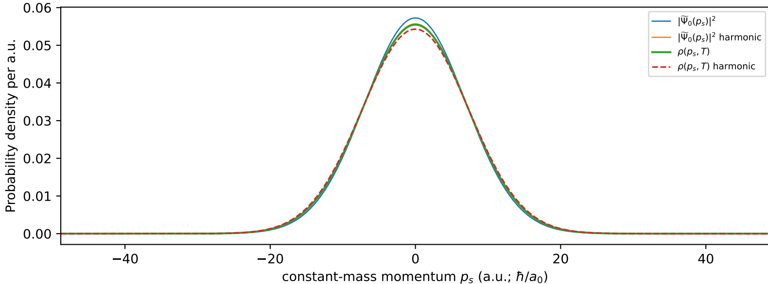
vib3 Momentum Distribution
