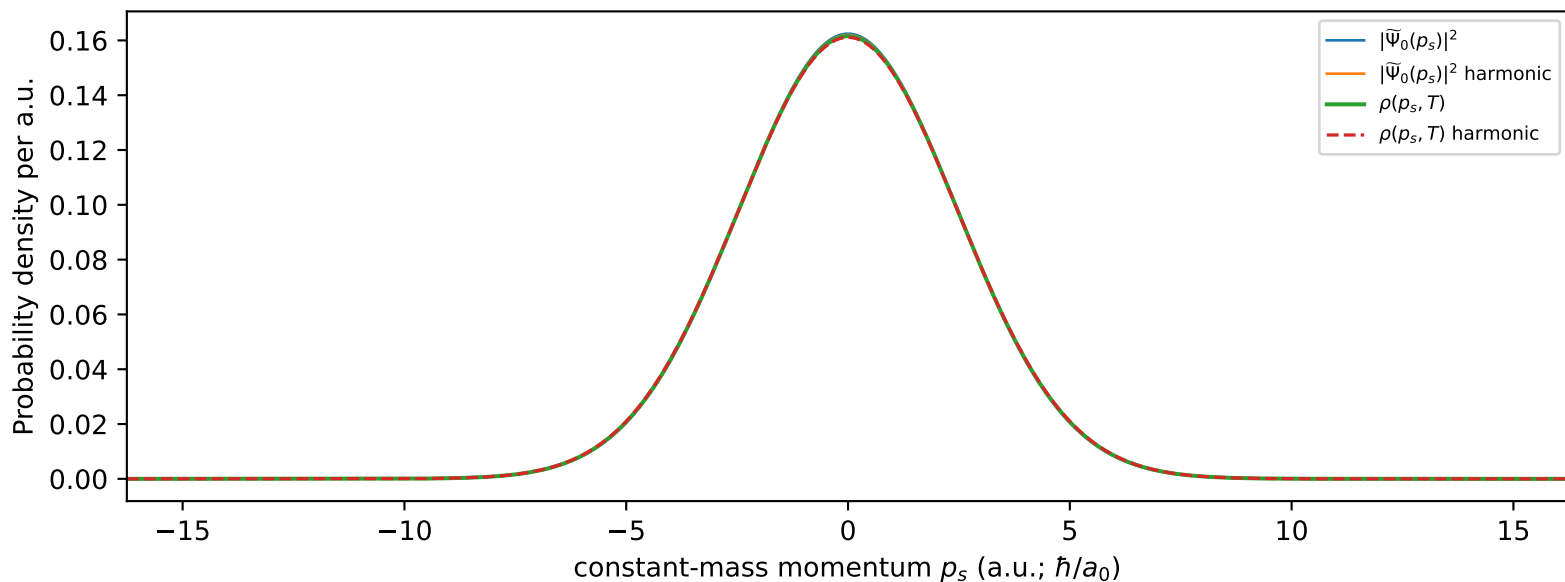
vib4 Momentum Distribution
