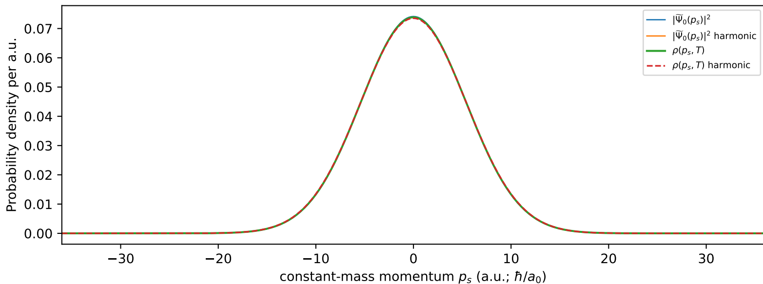
vib5 Momentum Distribution
