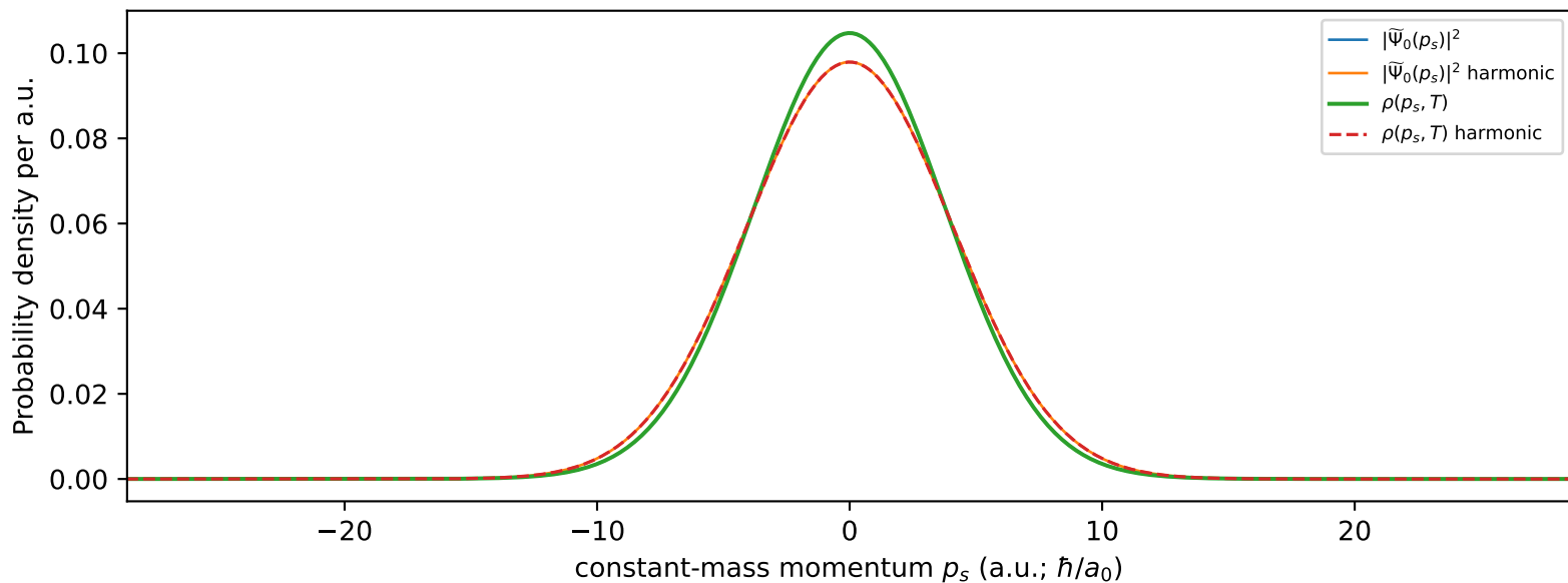
vib6 Momentum Distribution
