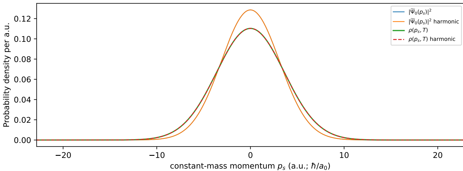
vib2 Momentum Distribution
