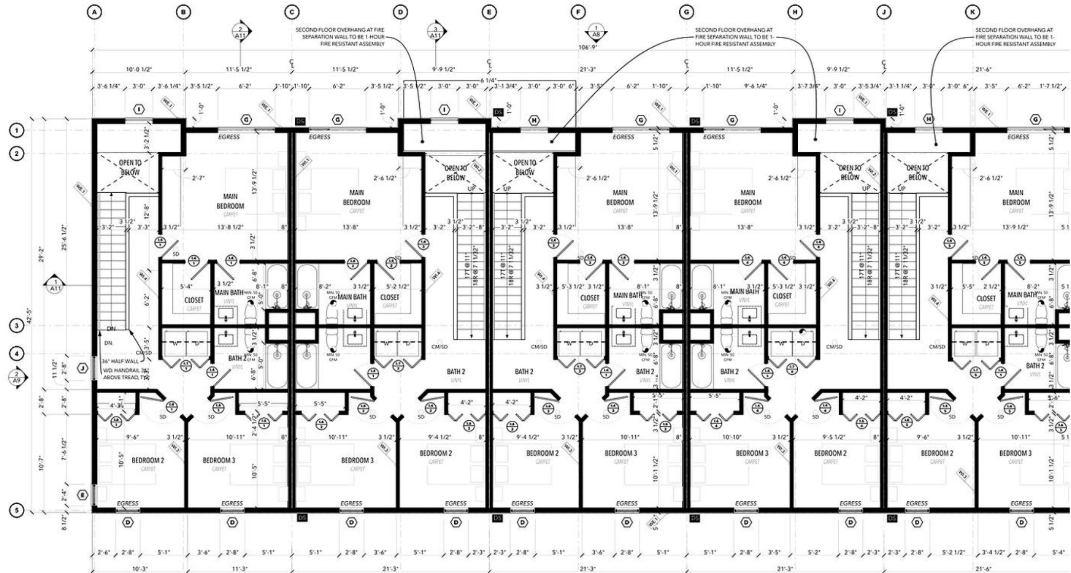
SECOND FLOOR SCALE: 1/4" = 1'-0"
