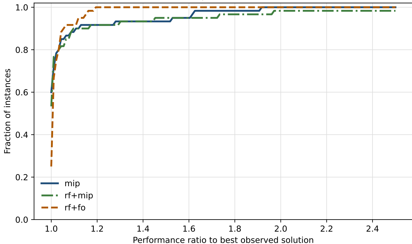
Performance profile at 600 seconds
