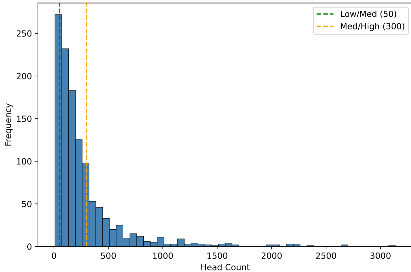
Crowd Count Distribution
