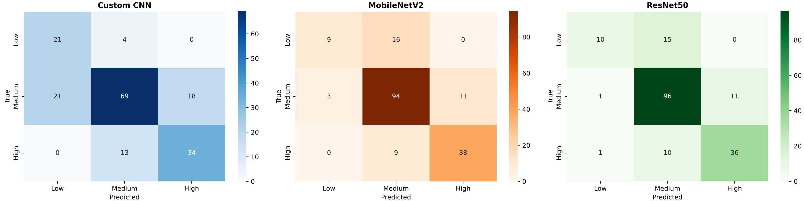
Figure 4: Confusion Matrices
