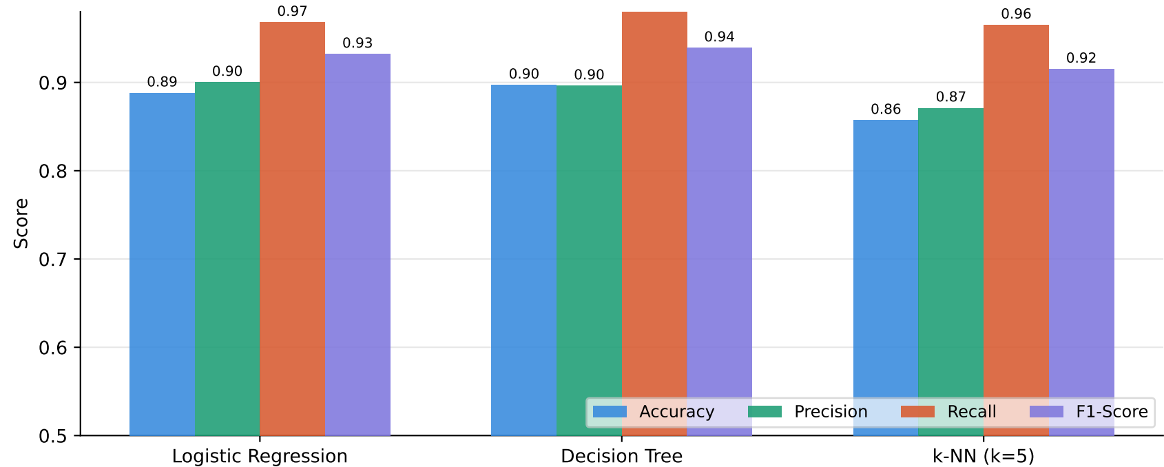
Fig. 1 — Baseline model performance (Loan Prediction Dataset 2025)
