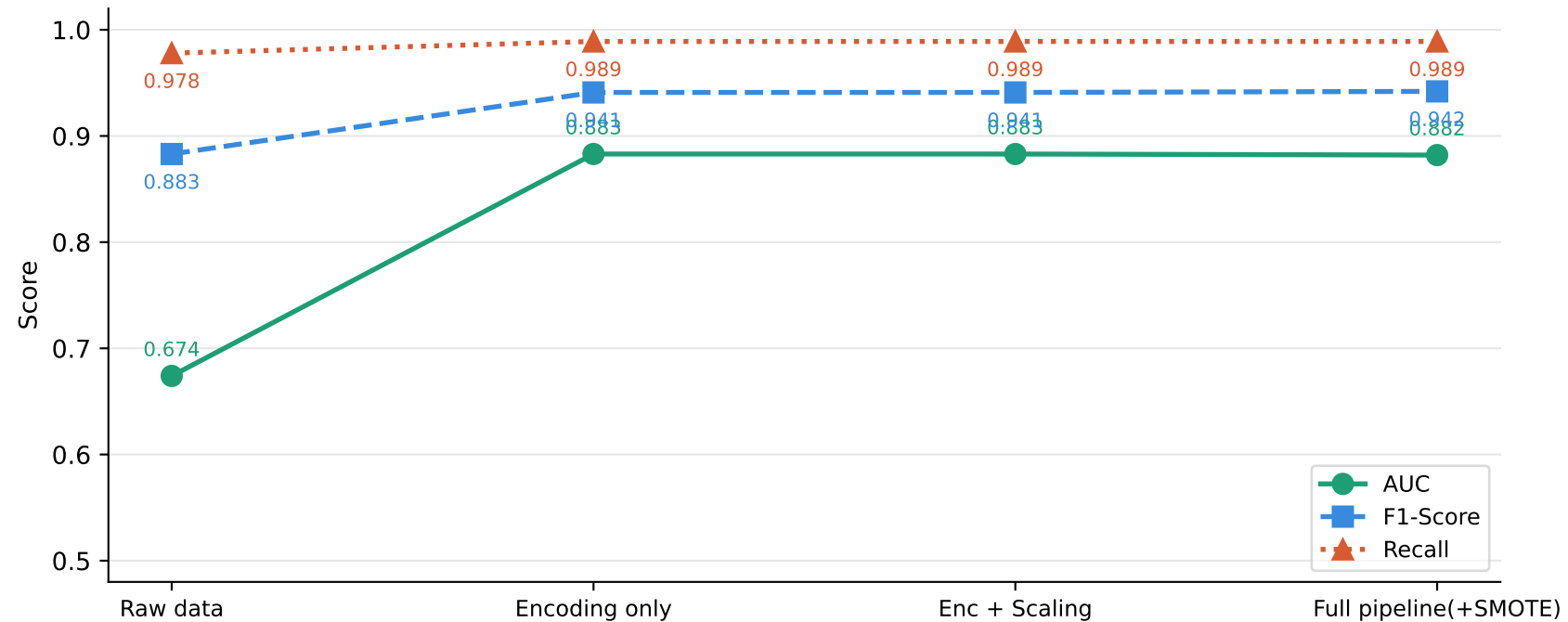
Fig. 3 — Incremental gains from preprocessing pipeline (XGBoost)
