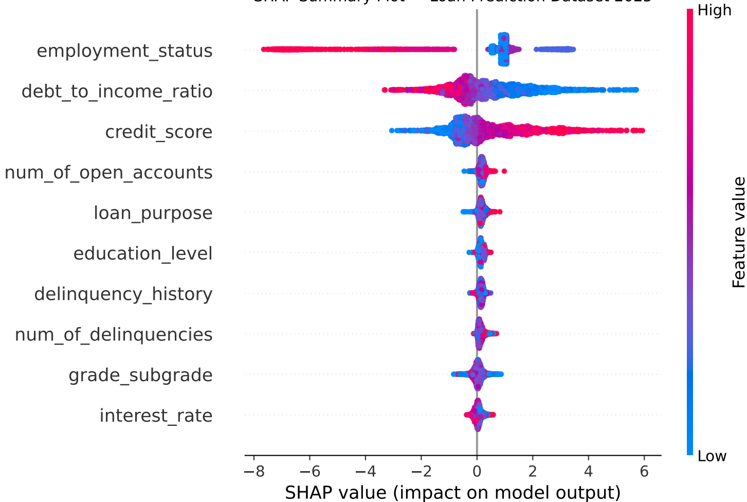
SHAP Summary Plot — Loan Prediction Dataset 2025
