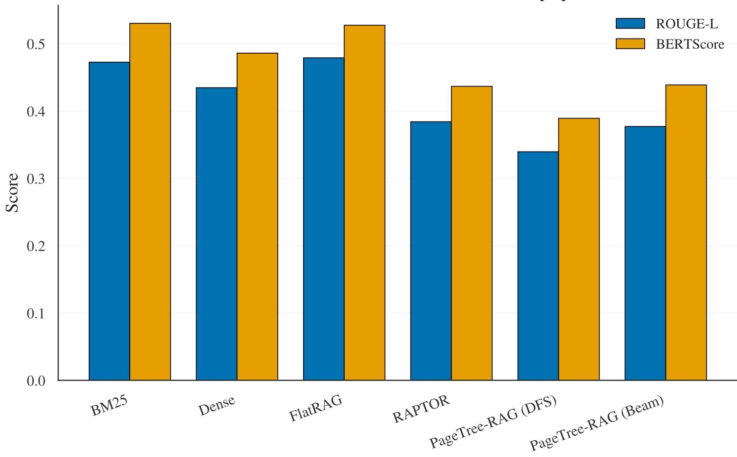
Main results: ROUGE-L and BERTScore by system
