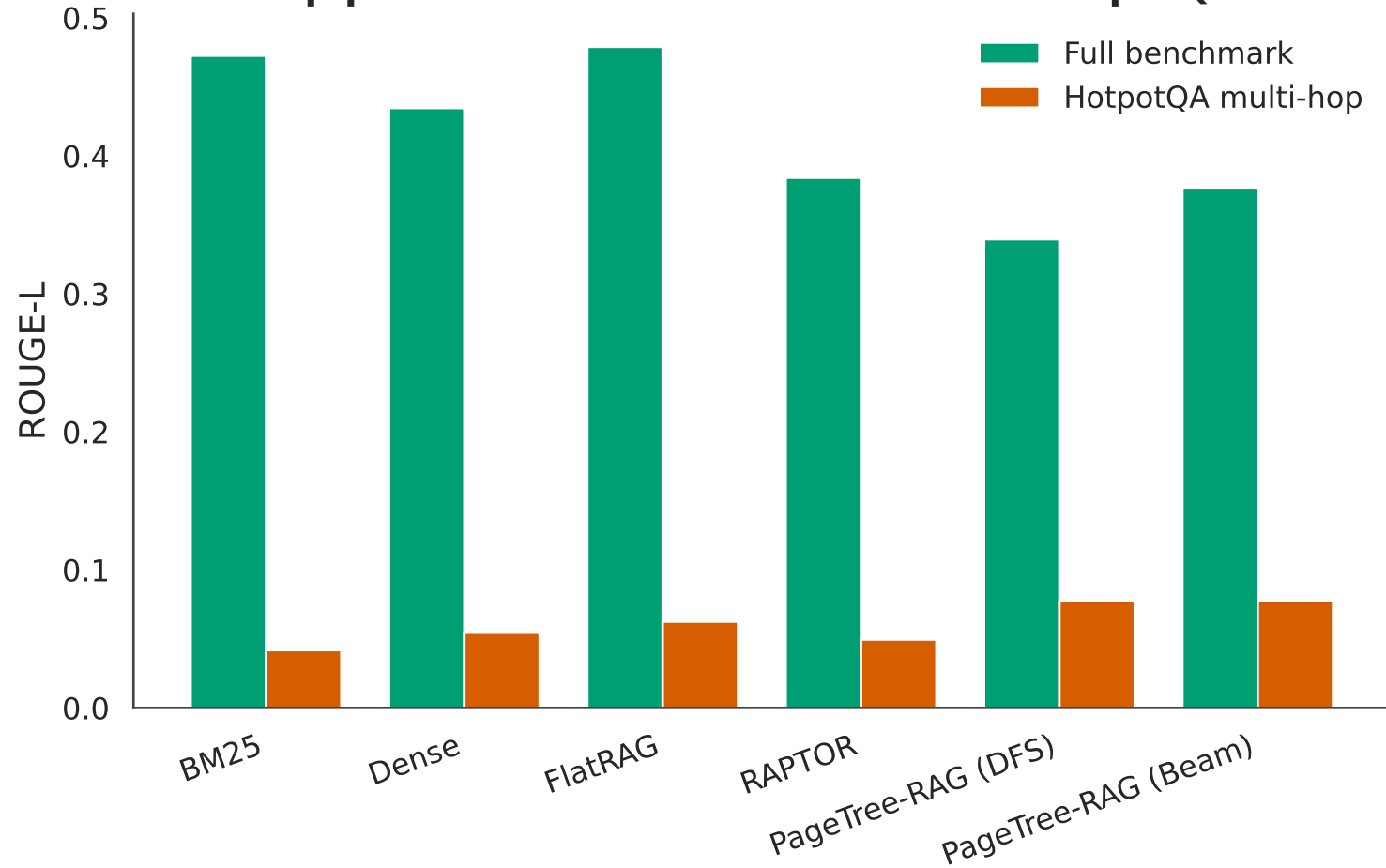
Multi-hop performance: full benchmark vs HotpotQA subset
