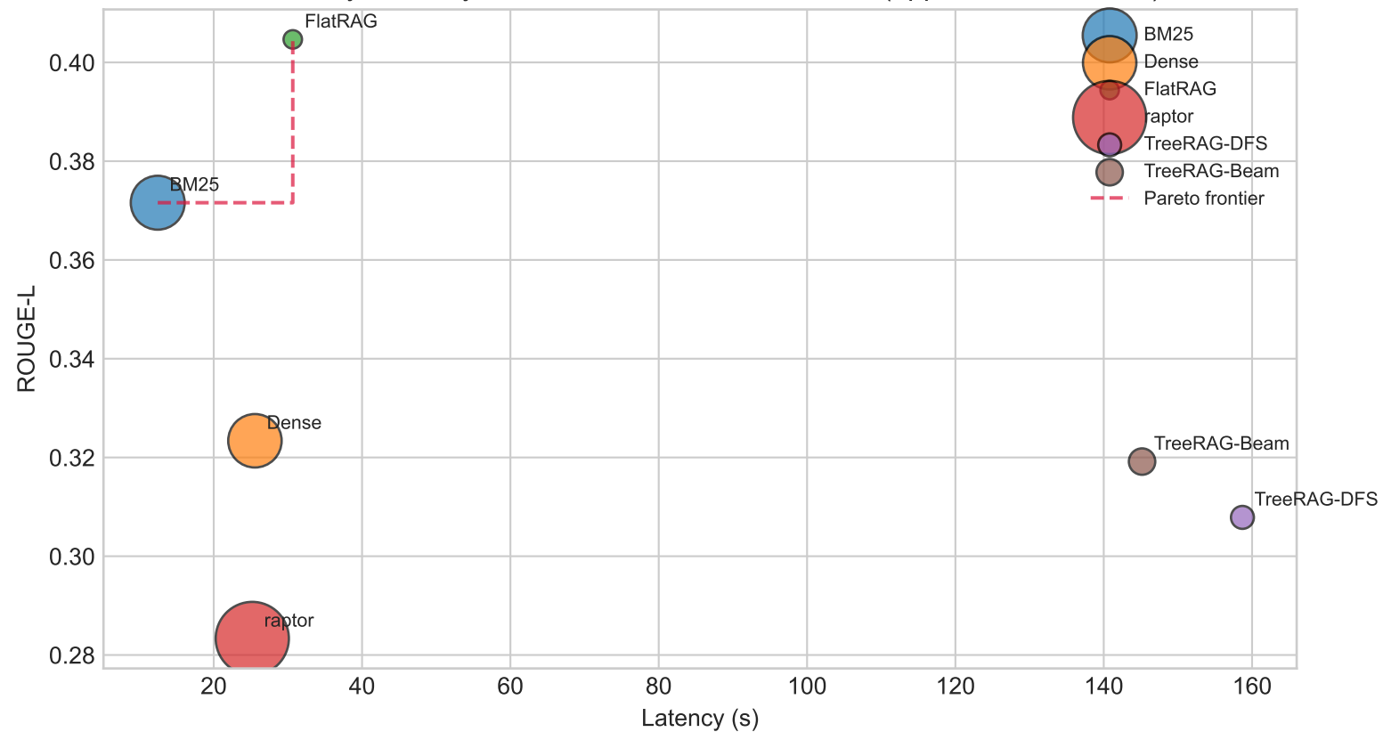
Efficiency: Latency vs ROUGE-L — Pareto frontier (upper-left dominates)
