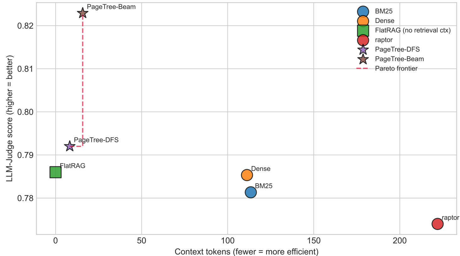
Efficiency: context tokens vs LLM-Judge fewer tokens, higher quality (upper-left dominates)
