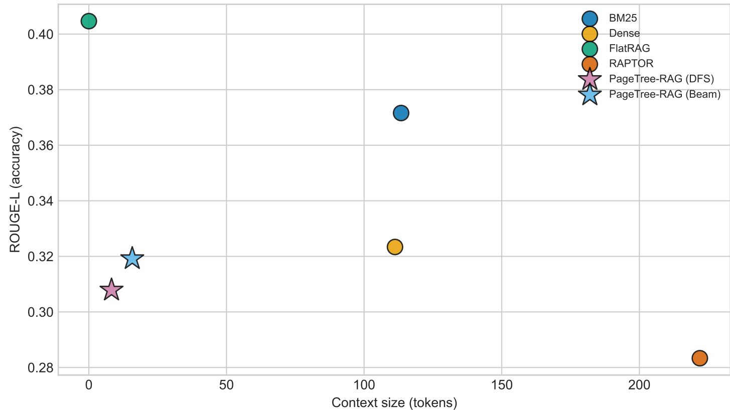
Accuracy vs context size — Pareto frontier (upper-left dominates)
