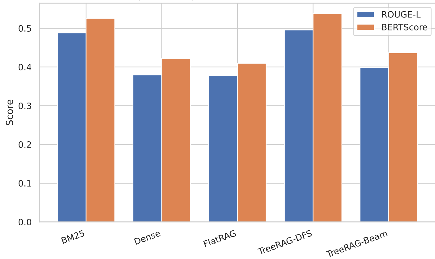
System comparison: ROUGE-L vs BERTScore
