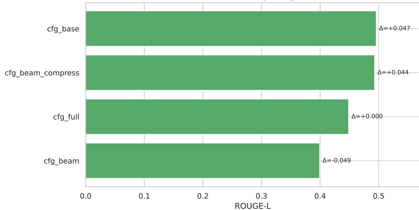
Ablation: ROUGE-L by configuration
