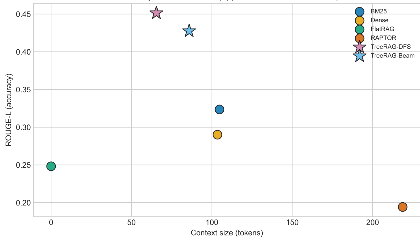
Accuracy vs context size (upper-left Pareto-dominates)
