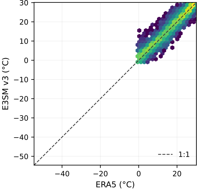
(d1) Global: r = 0.994
