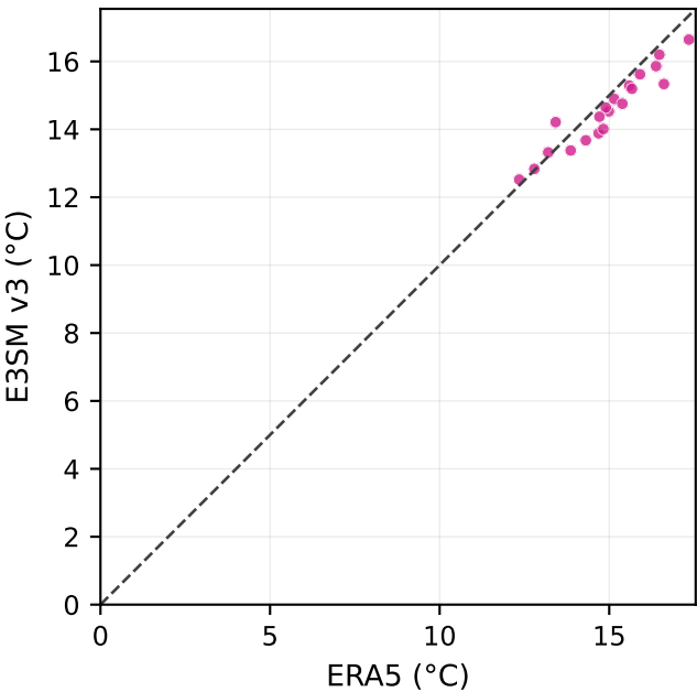
(d2) TVA: r = 0.952 ( n=20 )
