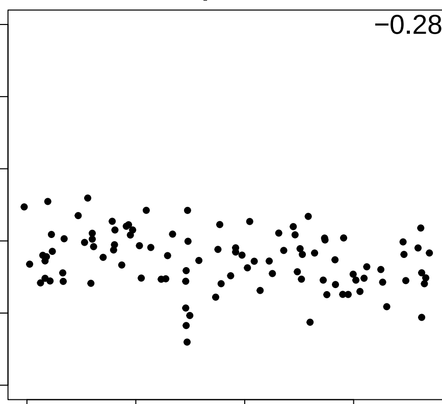
Dispersal
