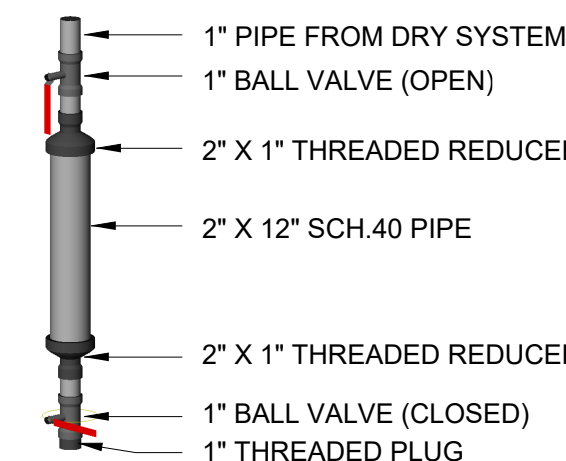
DRUM DRIP DETAIL
